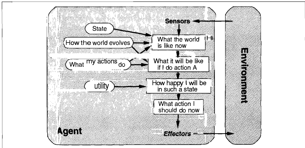
Figure 2.12 A complete utility-based agent.
