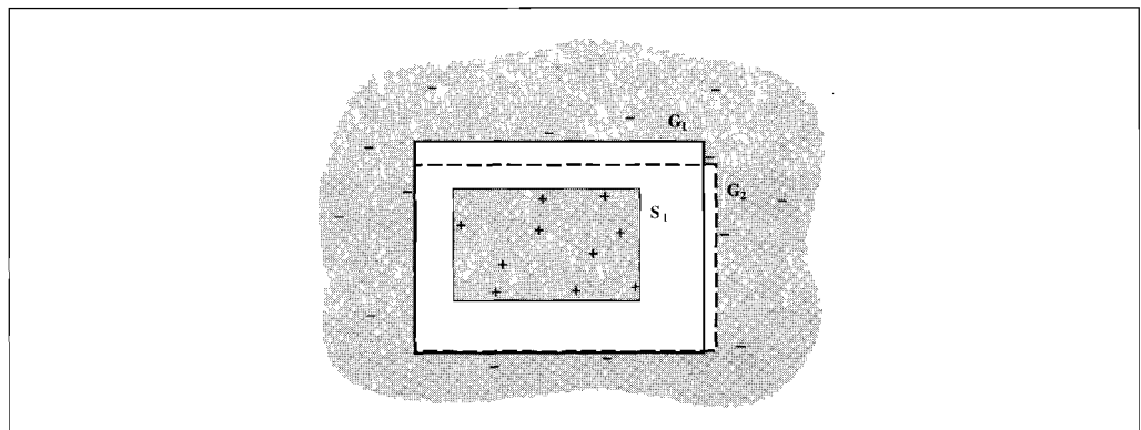
Figure 18.14 The extensions of the members of G and S . No known examples lie in between.
