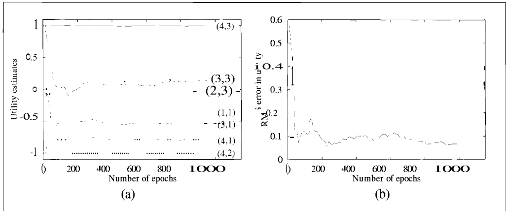
Figure 20.4 The LMS learning curves for the 4 \times 3 world shown in Figure 20.1. (a) The utility estimates of the states over time. (b) The RMS error compared to the correct values.
