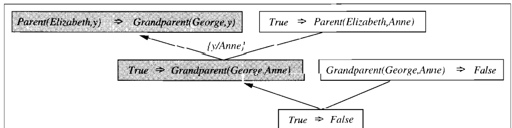
Figure 21.6 Early steps in an inverse resolution process. The shaded clauses are generated by inverse resolution steps.
