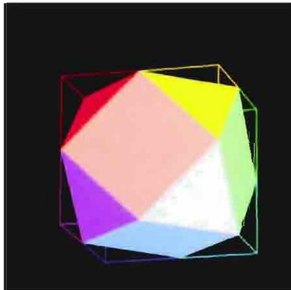
3.5 Figure 1 Partitioning of 3-space into 16 regions.
