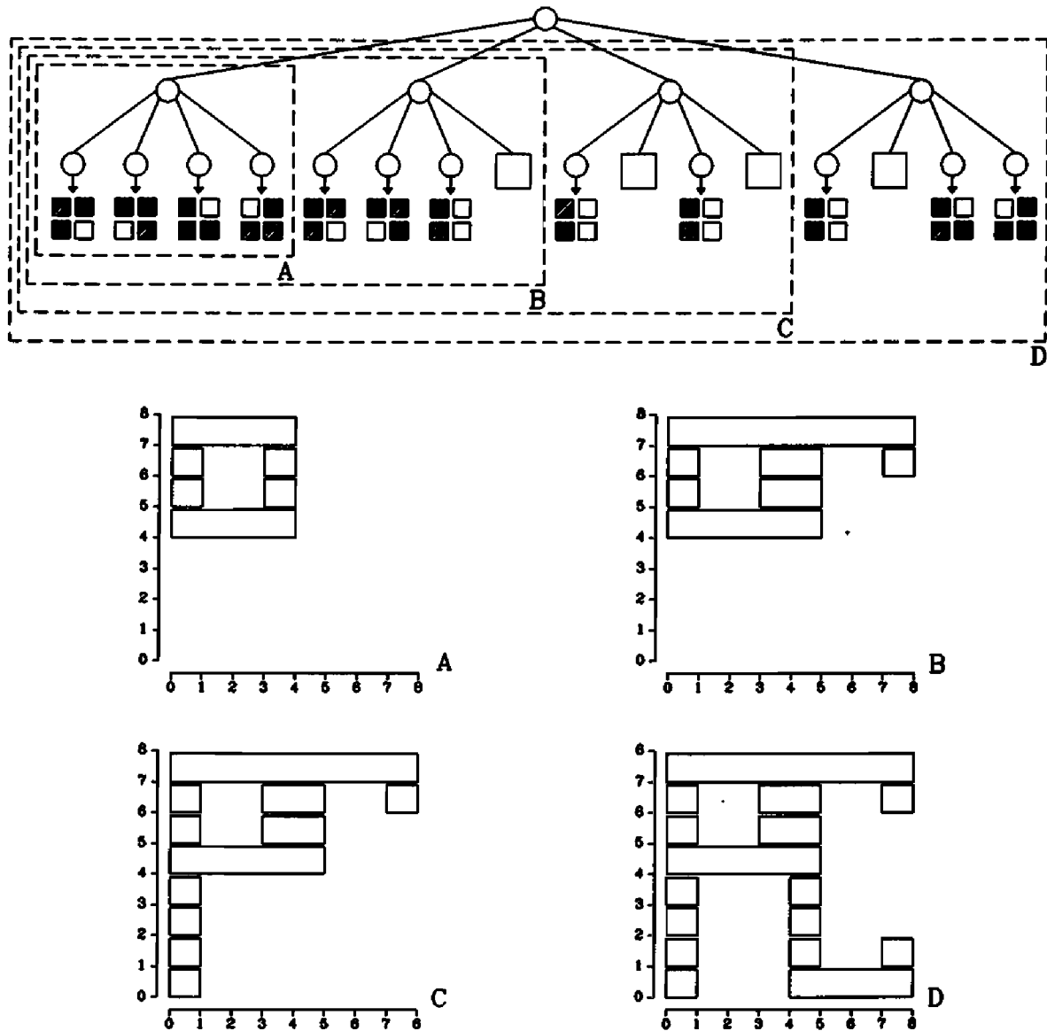
Figure 9. The making of the PCS data structure during the depth-first visit of the quadtree.
