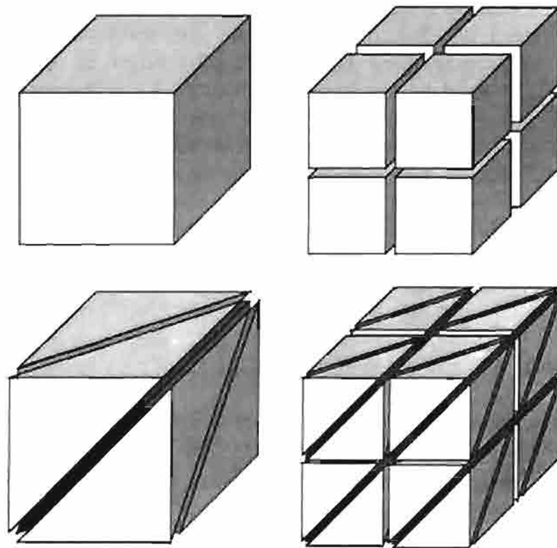
Figure 3. Symmetric subdivision from box subdivision.
