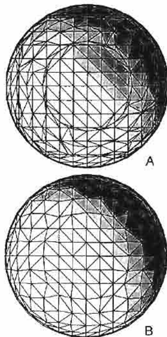
Figure 3. Two approximations to a sphere.
