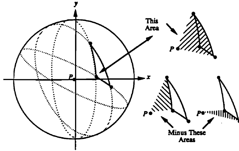
Figure 2. Projection of spherical triangle on equatorial plane.
