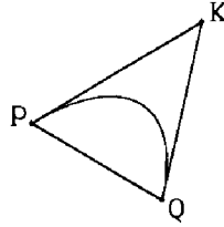
Figure 2 An elliptical arc and its control polygon.
