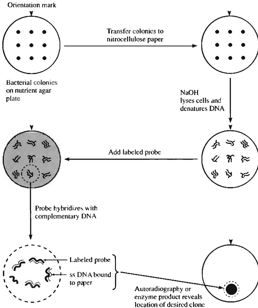
Fig. 13-8. The colony hybridization technique.
