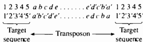
Fig. 12.15. Diagram of a simple transposon. Letters and numbers are used instead of nucleotides to make the repeats easier to read. Primed and unprimed symbols of the same kind (e.g., 3 and 3', d and d' ) represent complementary base pairs. The ends of a transposon consist of inverted repeats (represented by letters). Direct repeats of the target sequence (represented by numbers) flank the transposon. The dotted central region of simple transposons contains only genes necessary for translocation, but in complex transposons it may contain one or more additional genes.
