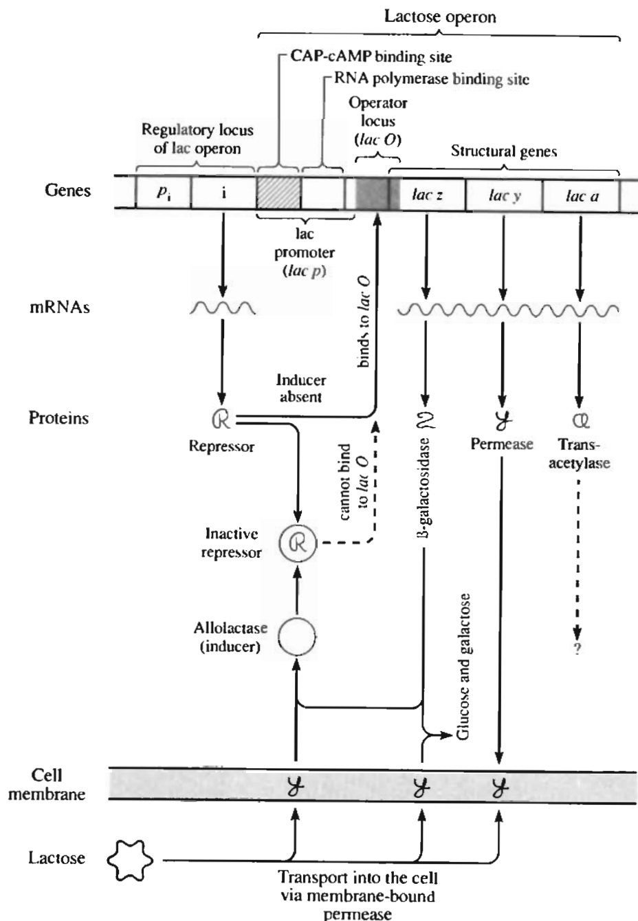
Fig. 12-12. Diagram of major elements controlling the lactose operon.
