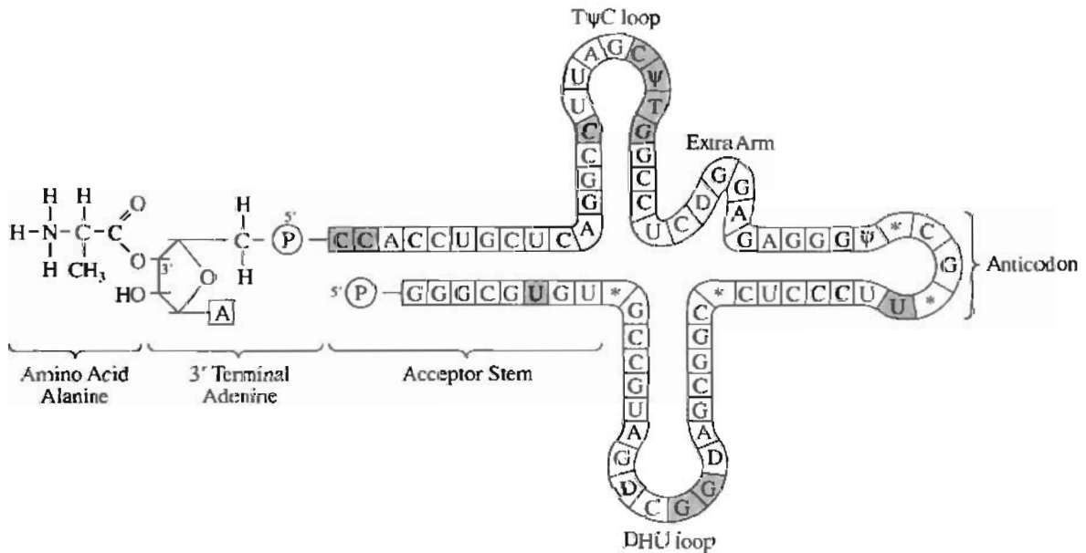
Fig. 11-8. A "cloverleaf model" of the yeast alanine transfer RNA molecule. All species of tRNA are about 75 ribonucleotides in length, with three major loops of unpaired bases. The middle loop contains the anticodon that can base pair with a codon in mRNA. The loop nearest the 3' end (called the T \psi C loop) is thought to interact with rRNA in the ribosome. There are several unusual bases (*) in tRNAs; pseudouridine ( \psi ) is one of them. The loop nearest the 5' end is called the DHU loop because it contains another unusual base, dihydrouridine (D). Enzymes in the nucleus modify the normal bases (A, U, C, G) in the preformed tRNA to create these unusual (rare) bases. All tRNAs end with CCA3'; the proper species of amino acid is attached to the terminal A by its cognate aminoacyl-tRNA synthetase enzyme. Some of the positions bearing identical bases in almost all tRNA species are indicated by shading.
