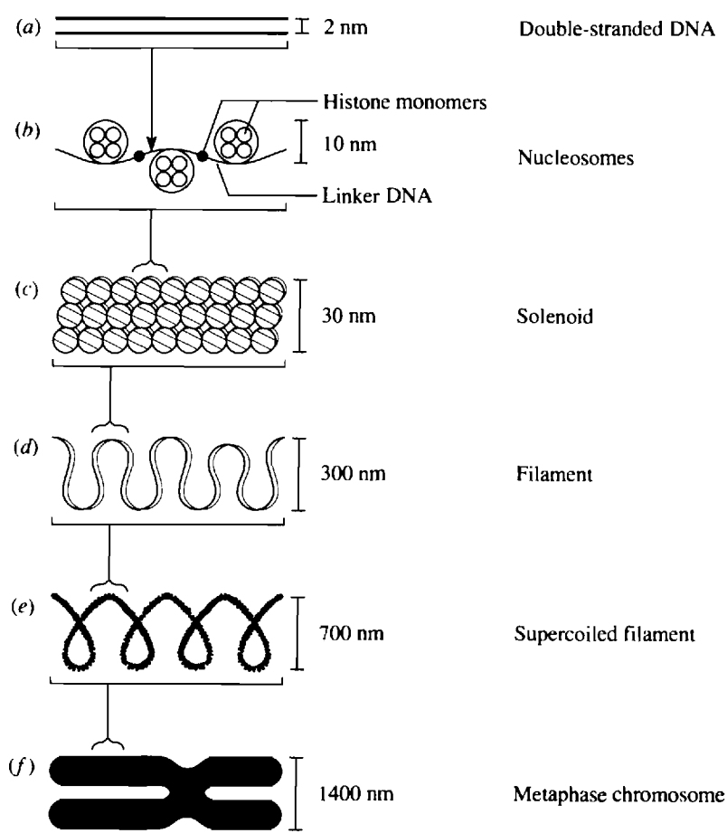
Fig. 14-1. Structural levels of organization hypothesized to occur during the condensation of a chromosome. (After J. D. Watson et al., 1987, Molecular Biology of the Gene , 4th ed., Benjamin/Cummings Publishing Company, Inc.).
