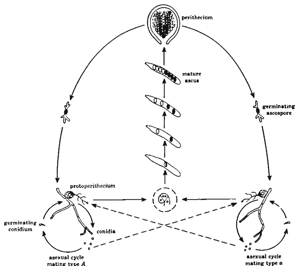
Fig. 6-3. Life cycle of Neurospora crassa .
