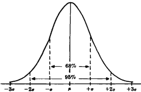
Fig. 9-2. A normal distribution.
