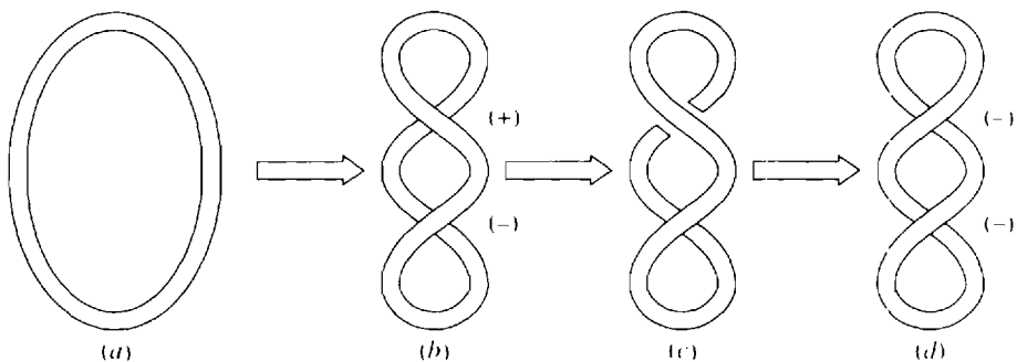
Fig. 12-2. A proposed mechanism whereby DNA gyrase "pumps" negative supercoiling into DNA. A relaxed, covalently closed, circular DNA molecule (a) is bent into a configuration for strand passage (b). DNA gyrase makes double-stranded cuts (c), holds onto the ends, passes an intact segment through the break, and reseals the break on the other side (d).
