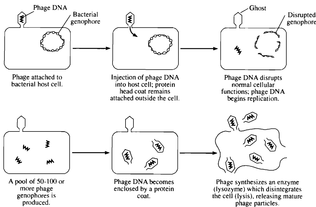
Fig. 12-16. Lytic life cycle of T-even phages.
