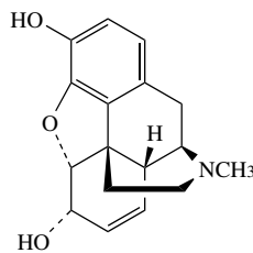
Morphine (Heroin, OHs = OCOCH 3 )
