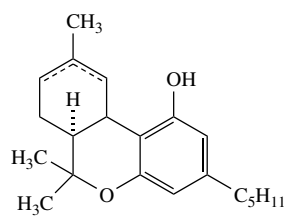
Δ 9 -Tetrahydrocannabinol (THC)
