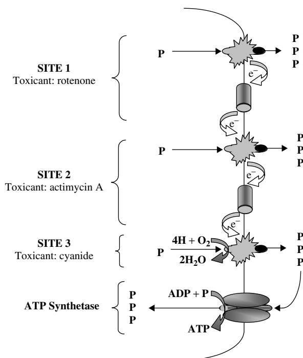
Figure 11.7 Electron ( e^- ) transport along the inner mitochondrial membrane resulting in the pumping of protons (P) out of the mitochondrial matrix. Protons are shuttled back into the matrix through the ATP synthetase complex where ATP is generated. Sites of toxicant action are indicated.
