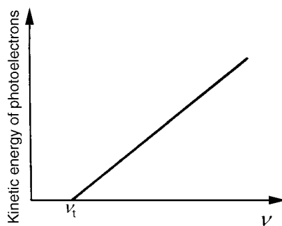
Figure 1.2 Variation of kinetic energy of photoelectrons with the frequency, \nu , of incident radiation
