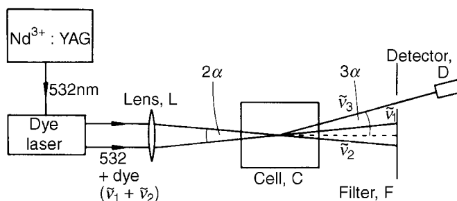
Figure 9.22 Experimental arrangement for coherent anti-Stokes Raman scattering
