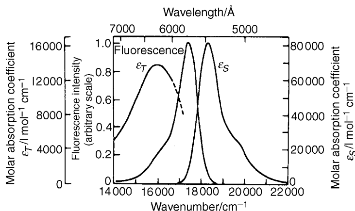
Figure 9.17 Absorption and fluorescence spectra of rhodamine B in methanol ( 5 \times 10^{-5} \text{ mol l}^{-1} ). The curve marked \epsilon_T is for the T_2 - T_1 absorption (process 8 in Figure 9.18) and that marked \epsilon_S for process 1. (Reproduced, with permission, from Dienes, A. and Shank, C. V., Chapter 4 in Creation and Detection of the Excited State (Ed. W. R. Ware), Vol. 2, p. 154, Marcel Dekker, New York, 1972)
