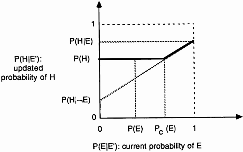
Figure 7.12: “Sufficiency-only” updating function.
