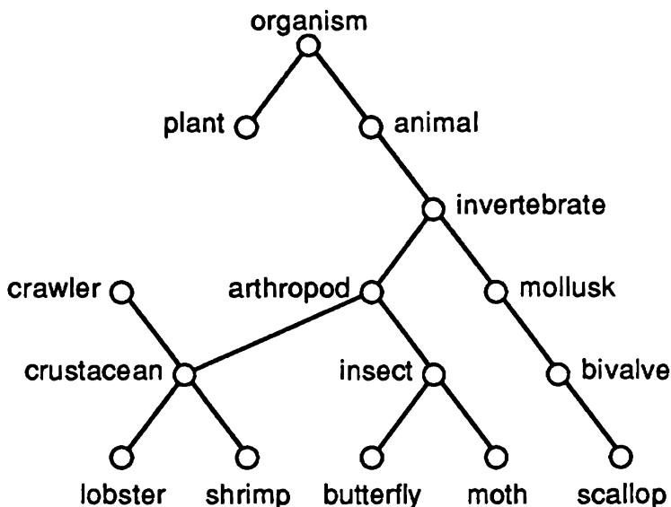
Figure 4.4: An ISA hierarchy for which the test (ISATEST 'LOBSTER 'ANIMAL 20) succeeds.
