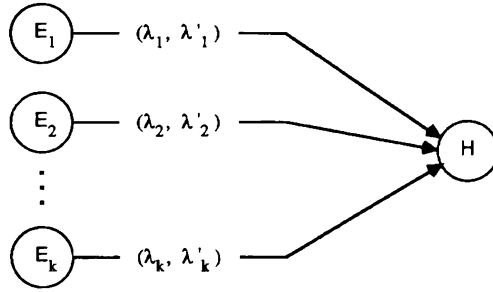
Figure 7.14: Combining independent evidence.
