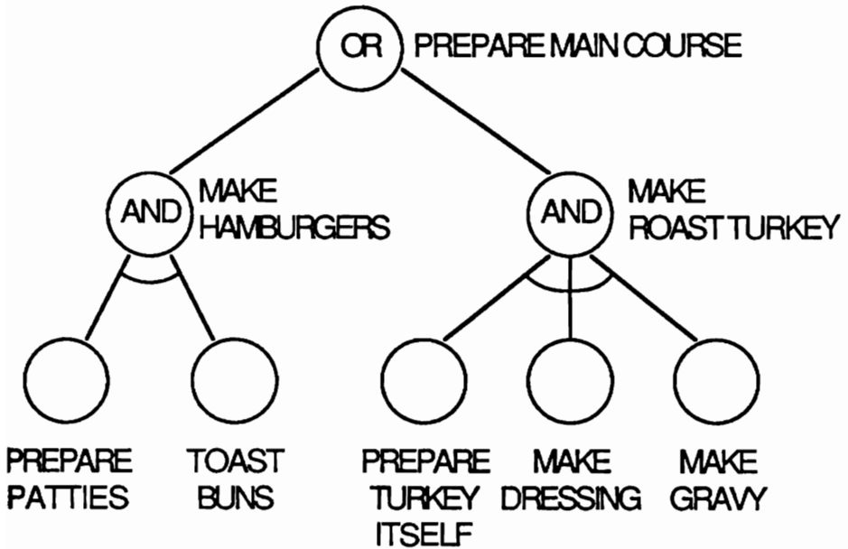
Figure 5.10: An AND/OR tree.
