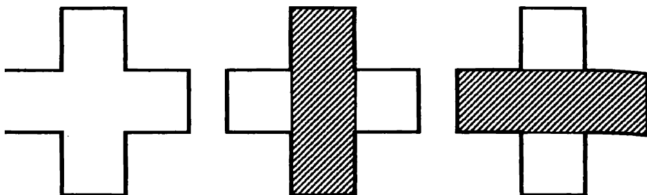
Figure 10.28: A shape having two convex kernels.
