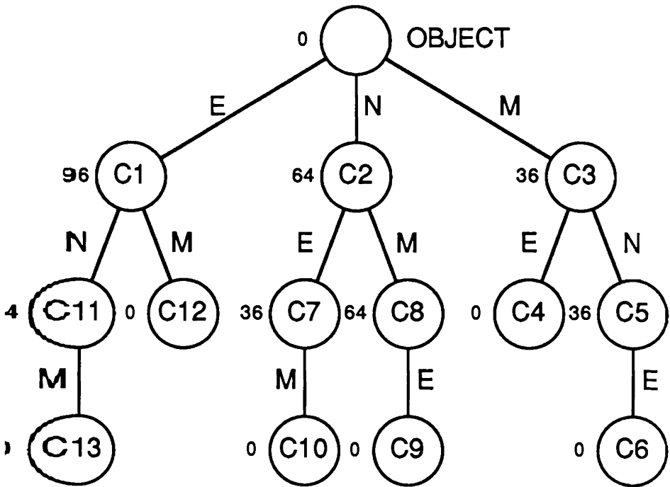
Figure 8.4: The space of concepts explored by the PYTHAGORUS program.
