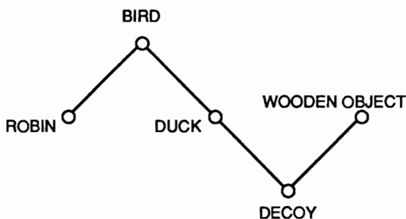
Figure 4.6: Multiple inheritance.
