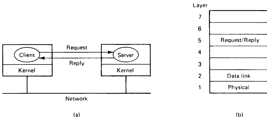
Fig. 2-7. The client-server model. Although all message passing is actually done by the kernels, this simplified form of drawing will be used when there is no ambiguity.
