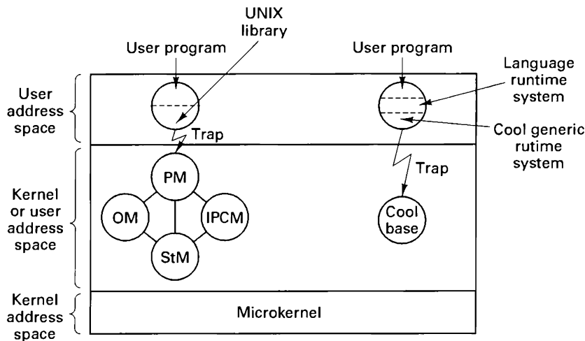
Fig. 9-26. Implementation of COOL.
