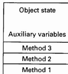
Fig. 6-34. An object.
