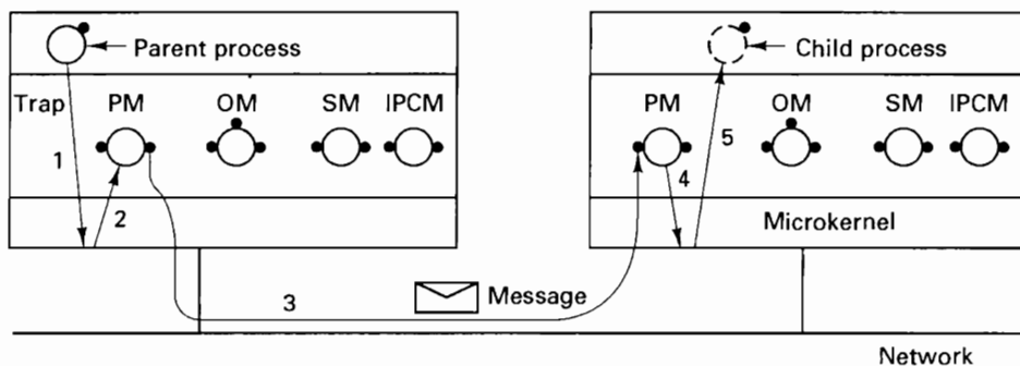
Fig. 9-21. Creating a process on a remote machine. The reply message is not shown.
