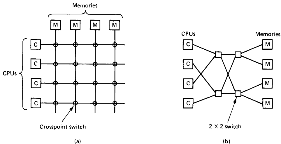
Fig. 1-6. (a) A crossbar switch. (b) An omega switching network.
