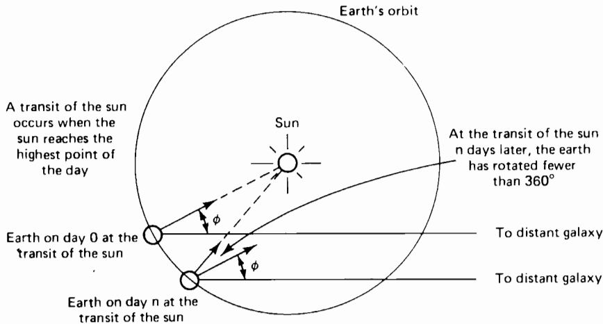
Fig. 3-3. Computation of the mean solar day.
