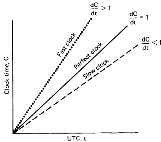
Fig. 3-5. Not all clocks tick precisely at the correct rate.
