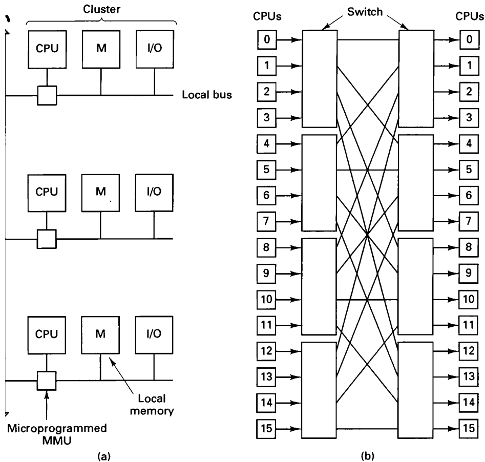
Fig. 6-9. (a) A simplified view of the Cm* system. (b) The BBN Butterfly. The CPUs on the right are the same as those on the left (i.e., the architecture is really a cylinder).
