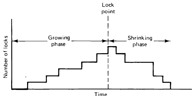
Fig. 3-21. Two-phase locking.
