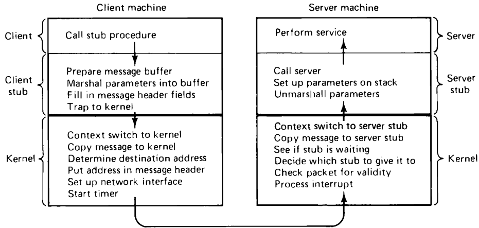
Fig. 2-26. Critical path from client to server.
