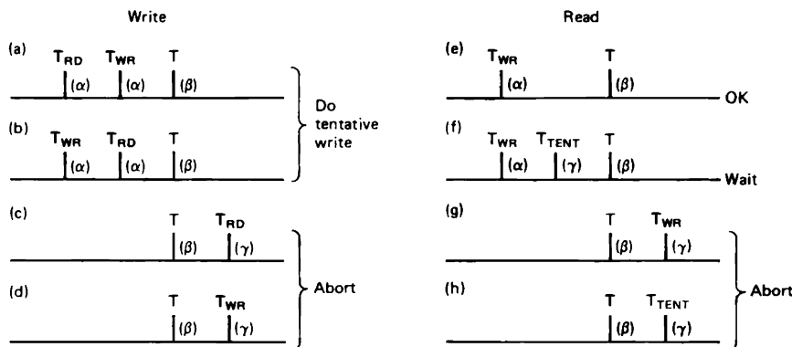
Fig. 3-22. Concurrency control using timestamps.
