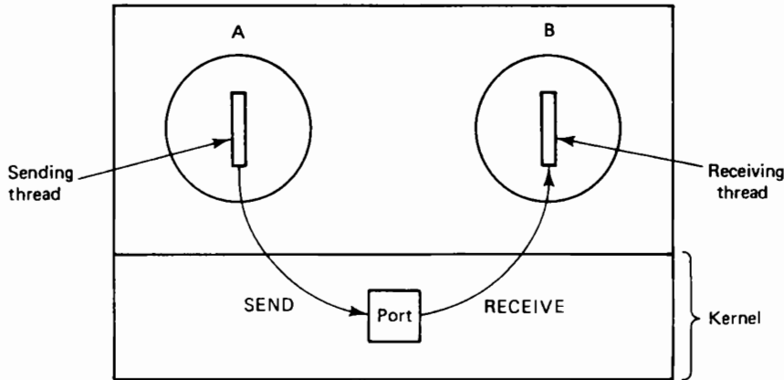
Fig. 8-14. Message passing goes via a port.
