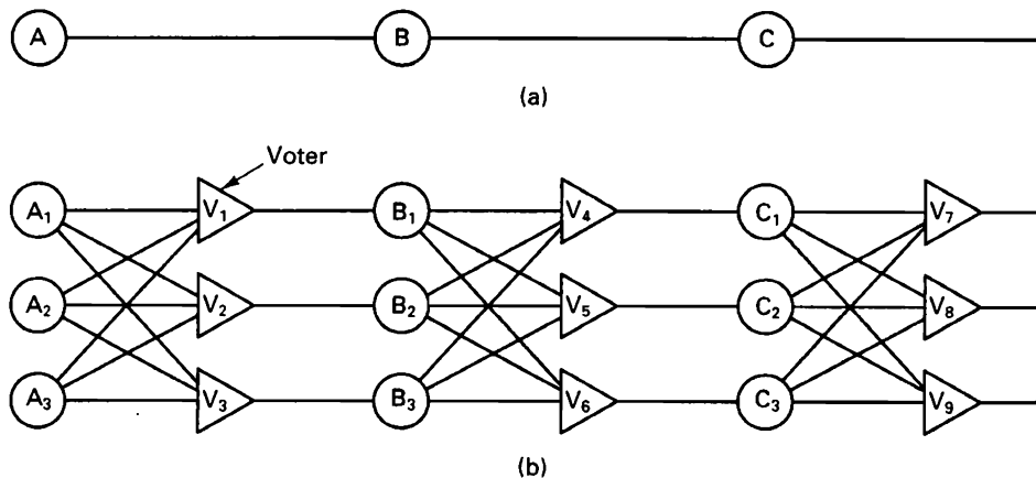
Fig. 4-21. Triple modular redundancy.
