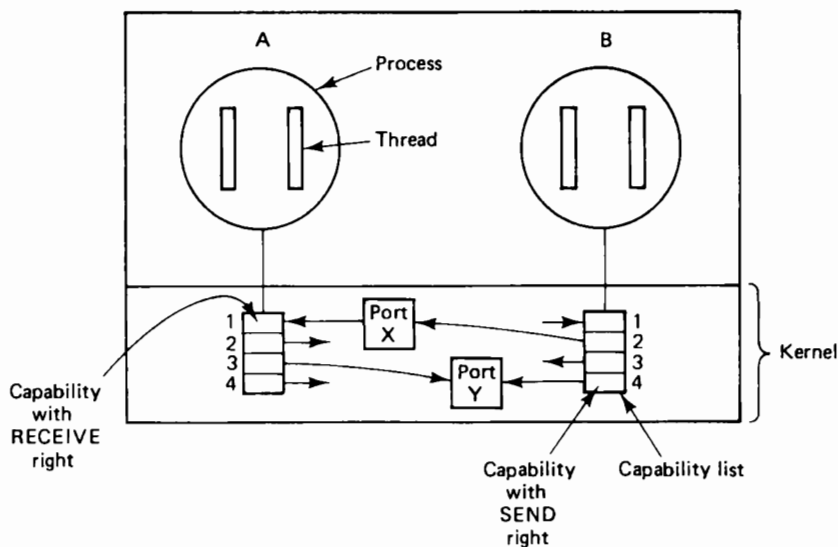
Fig. 8-15. Capability lists.
