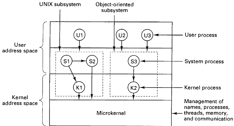
Fig. 9-1. Chorus is structured in layers, with a microkernel, subsystems, and user processes.
