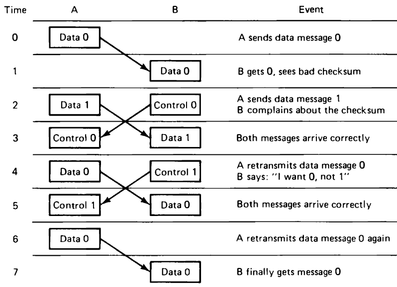
Fig. 2-3. Discussion between a receiver and a sender in the data link layer.
