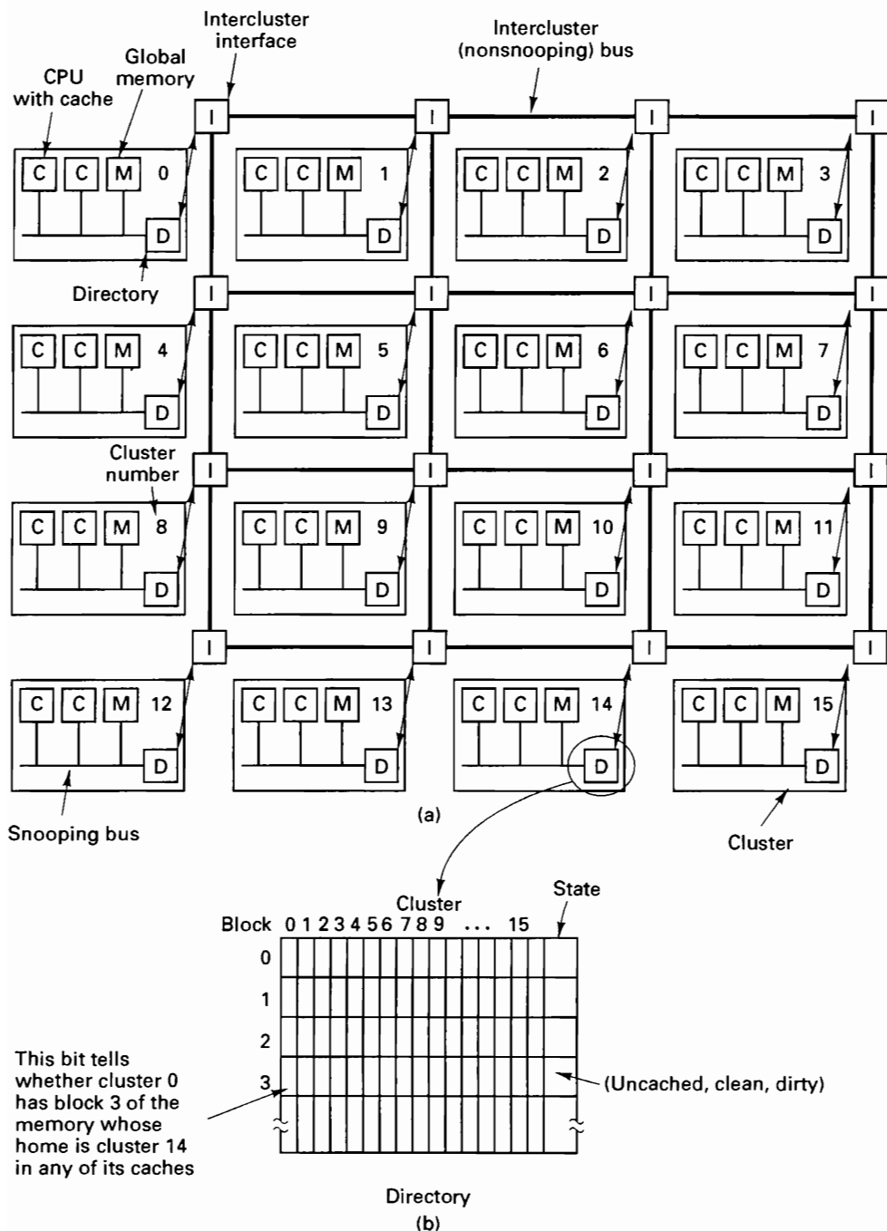
Fig. 6-7. (a) A simplified view of the Dash architecture. Each cluster actually has four CPUs, but only two are shown here. (b) A Dash directory.
