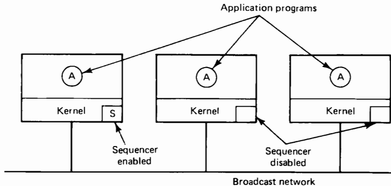
Fig. 7-11. System structure for group communication in Amoeba.
