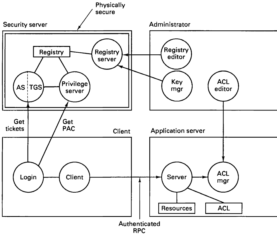
Fig. 10-26. Major components of the DCE security system for a single cell.
