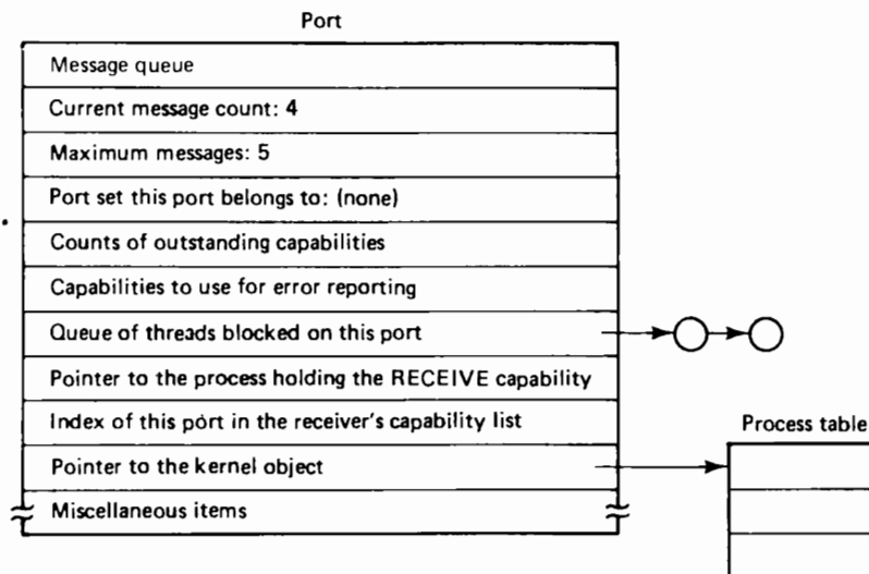
Fig. 8-13. A Mach port.
