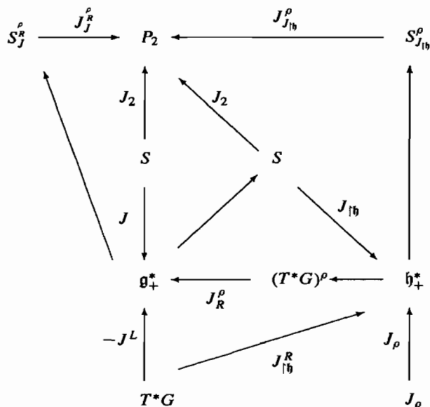
FIGURE 9. Marsden-Weinstein reduction in stages: S_J^\rho \simeq S_{J|_{\mathfrak{h}}}^\rho
