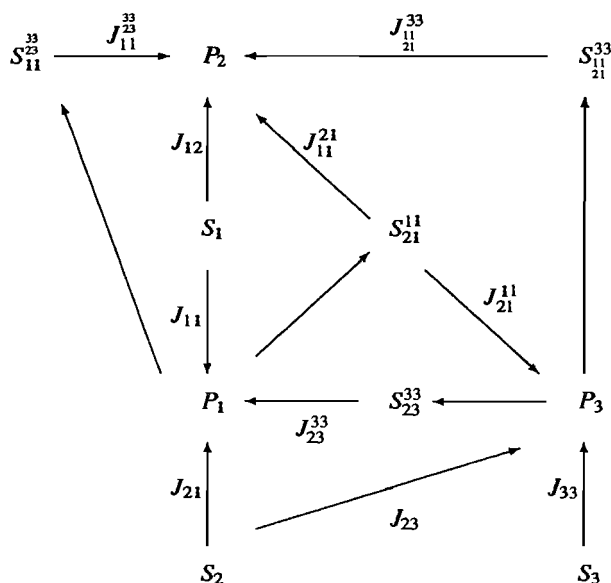
FIGURE 7. Reduction in stages: S_{21}^{33} \simeq S_{11}^{33} and J_{21}^{33} \simeq J_{11}^{33}
