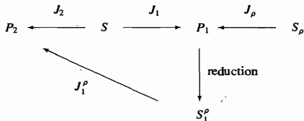
FIGURE 1. Special symplectic reduction; S_1^\rho := S_{J_1}^\rho etc.
