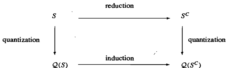
FIGURE 15. Constrained quantization: Q is some quantization procedure
