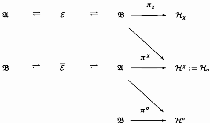
FIGURE 12. Quantum imprimitivity theorem: \mathcal{H}^\sigma \simeq \mathcal{H}_X and \pi^\sigma \simeq \pi_X
