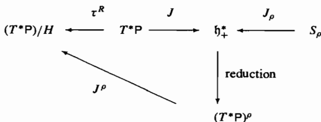
FIGURE 3. Kazhdan-Kostant-Sternberg reduction
