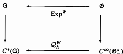
FIGURE 1. Groupoids and algebroids in quantization
