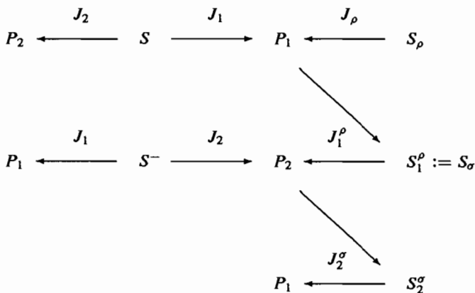
FIGURE 2. Classical imprimitivity theorem: S_2^\sigma \simeq S_\rho and J_2^\sigma \simeq J_\rho
