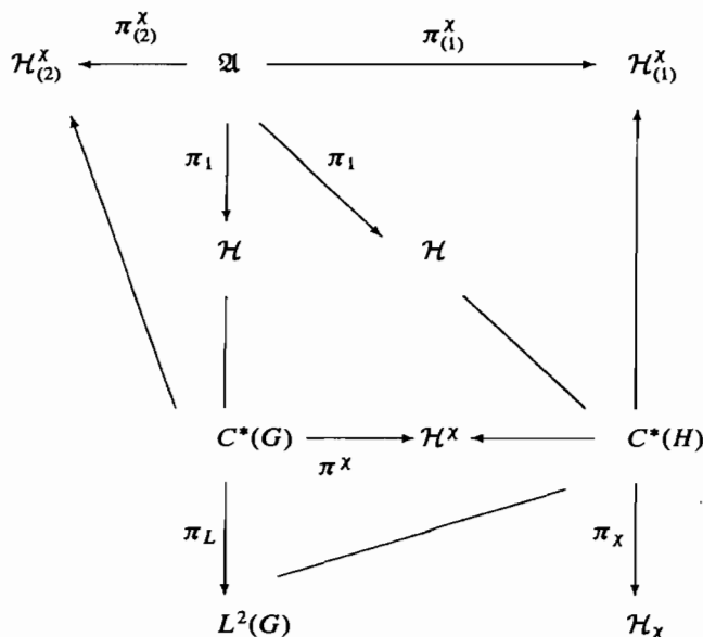
FIGURE 14. Quantum Marsden–Weinstein reduction in stages: \mathcal{H}_{(1)}^X \simeq \mathcal{H}_{(2)}^X and \pi_{(1)}^X \simeq \pi_{(2)}^X
