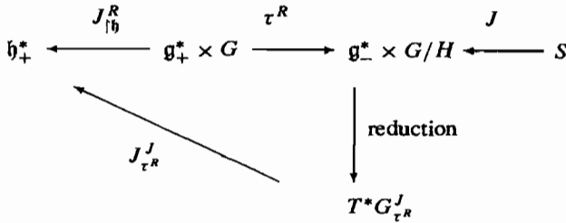
FIGURE 5. T^*G_{\tau^R}^J \simeq J_{(2)}^{-1}([e]_H)/\mathcal{N}_{G/H} and J_{\tau^R}^J \simeq [-J_{|\mathfrak{h}}]_H
