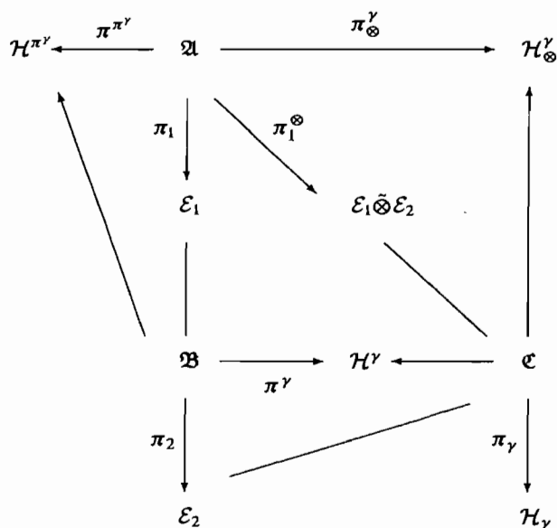
FIGURE 13. Rieffel induction in stages: \mathcal{H}^{\pi^\gamma} \simeq \mathcal{H}_\otimes^\gamma and \pi^{\pi^\gamma} \simeq \pi_\otimes^\gamma
