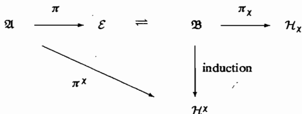
FIGURE 11. Rieffel induction
