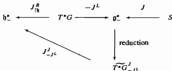
FIGURE 8. \widetilde{T^*G}_{-J^L}^J \simeq S and J_{-J^L}^J \simeq J_{|\mathfrak{h}}
