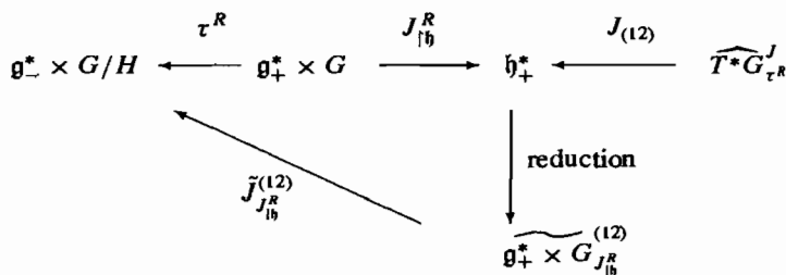
FIGURE 6. Classical imprimitivity: \widetilde{g_+^* \times G_{J_{|h}^R}^{(12)}} \simeq S and \widetilde{J_{J_{|h}^R}^{(12)}} \simeq J
