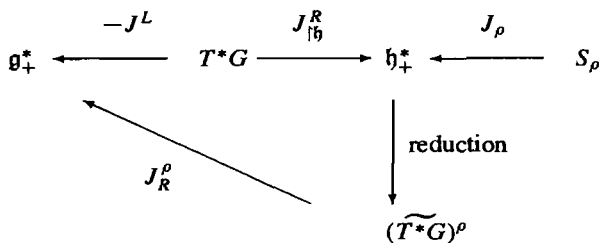
FIGURE 4. The reduced space (\widetilde{T^*G})^\rho
