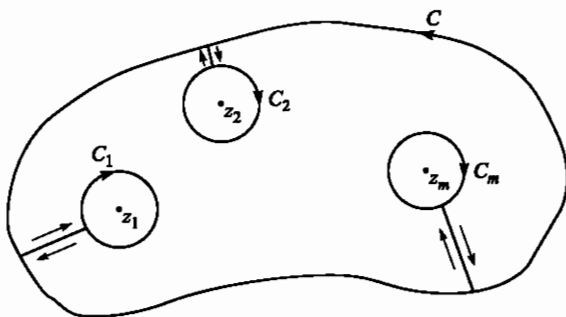
Figure 6.15. Residue theorem.
