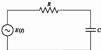
Figure 2.3. RC circuit.
