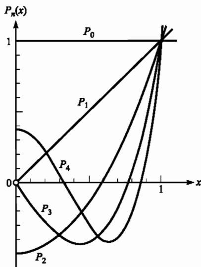
Figure 7.1. Legendre polynomials.
