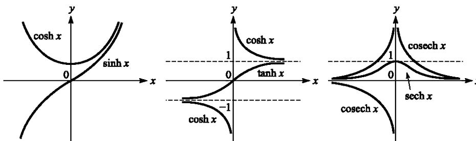
Figure A1.2. Hyperbolic functions.
