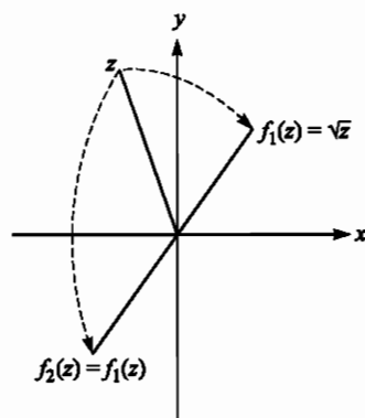
Figure 6.4. The mapping function w = \sqrt{z} .
