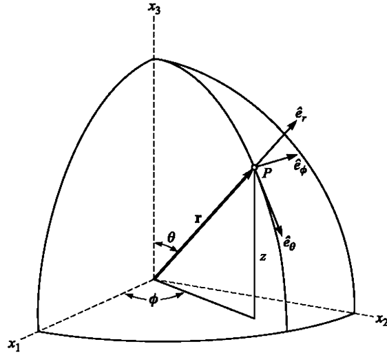
Figure 1.18. Spherical coordinates.
