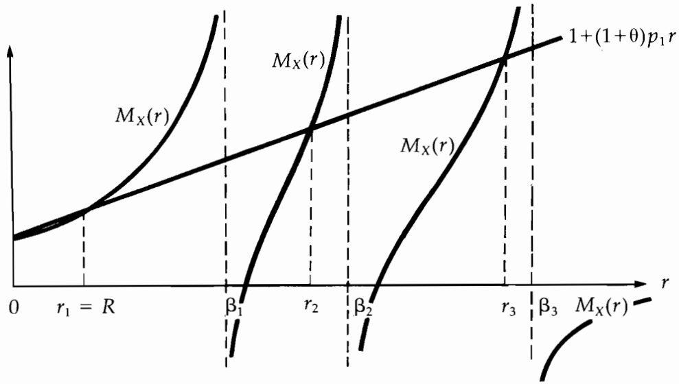
FIGURE 13.6.2 The Solution of (13.6.14) for n = 3
