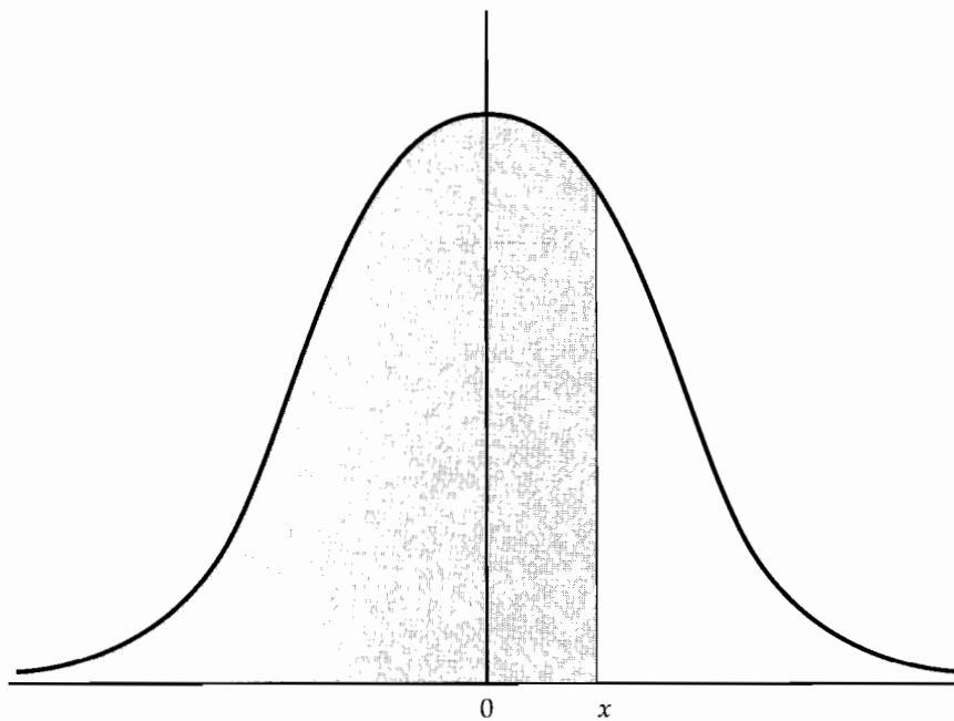
Normal Distribution
