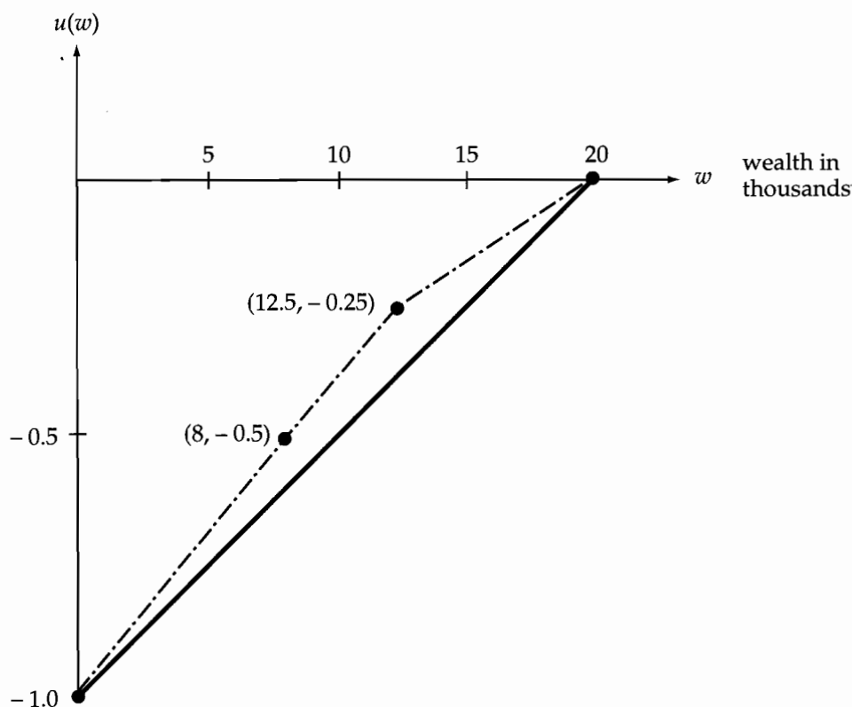
FIGURE 1.2.1 Determination of a Utility Function
