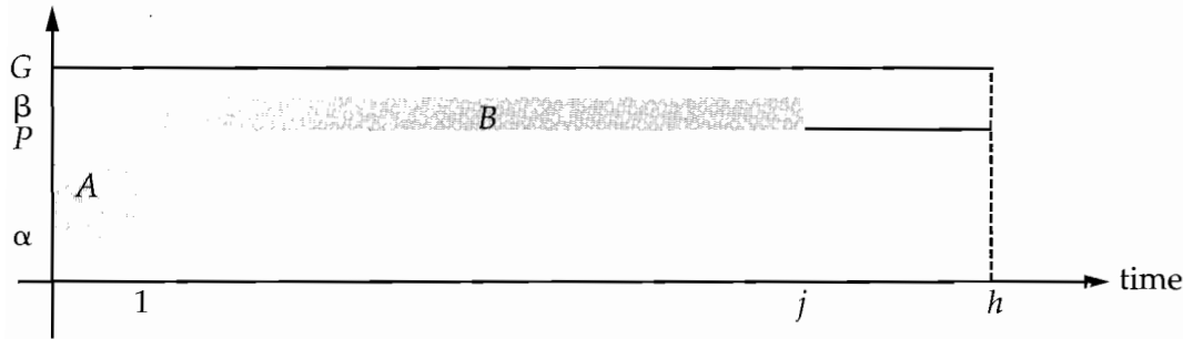
FIGURE 16.6.1 Premiums in a Modified Reserve Method
