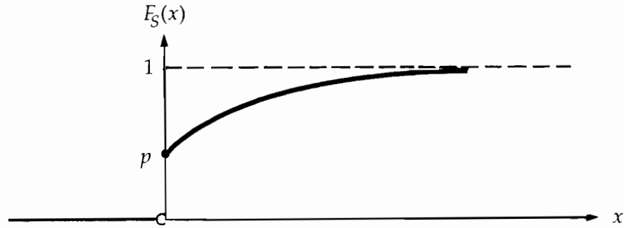
FIGURE 12.2.1 Graph of F_S(x)
