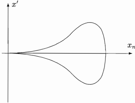
Figure 2: An exterior cusp
