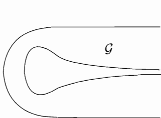
Figure 1a: A domain with singular point at infinity
