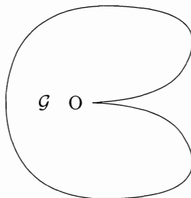
Figure 1b: A domain with singular point O
