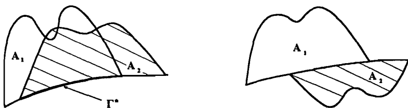
A_1 and A_2 are externally contact A_1 and A_2 are not externally contact
