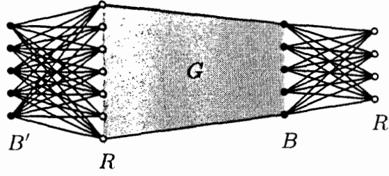
Figure 2.3: The graph G_k .
