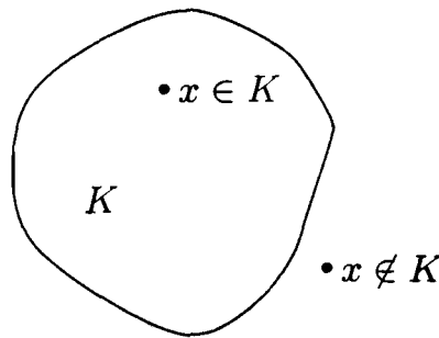
Figure 6.1: Oracle for K .
