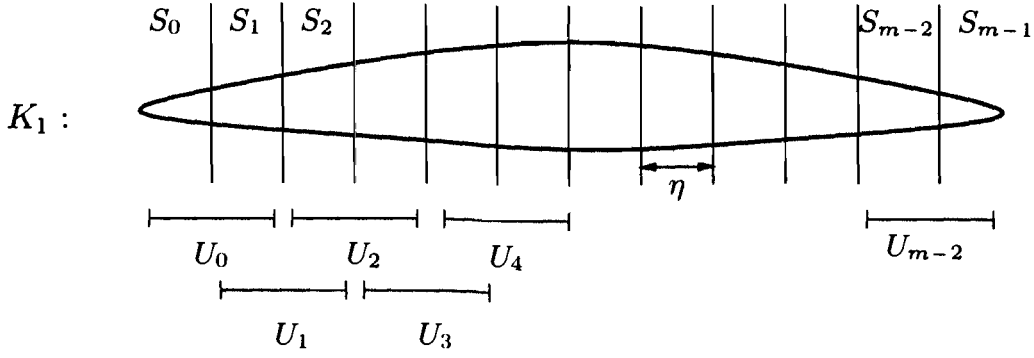
Figure 6.5: Partitioning of K_1
