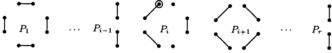
Figure 5.3: The corresponding encoding \eta_t(X, Y) .
