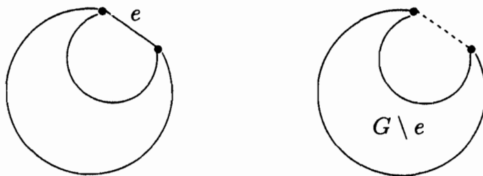
Figure 1.4: Orient e according to the condition of Lemma 1.13.
