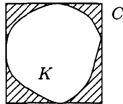
Figure 6.2: Sampling by “direct” Monte Carlo.
