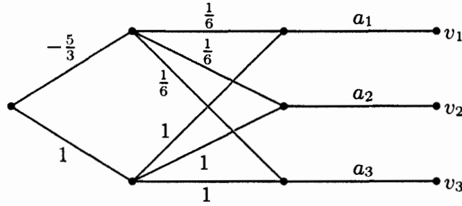
Figure 2.1: The graph H .
