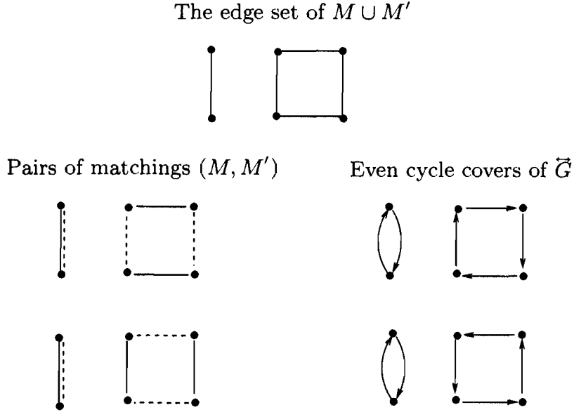
Figure 1.2: Bijection between pairs of matchings in G and even cycle covers of \vec{G} .
