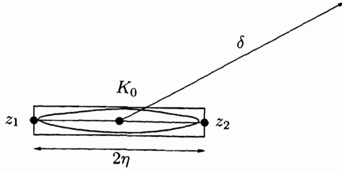
Figure 6.6: “Needle like” body K_0
