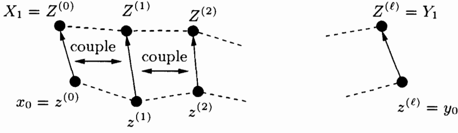
Figure 4.6: Extending a coupling along a shortest path
