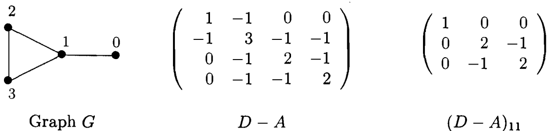
Figure 1.1: Example illustrating Theorem 1.1.
