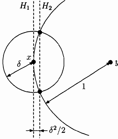
Figure 6.3: Bounding the volume of intersection
