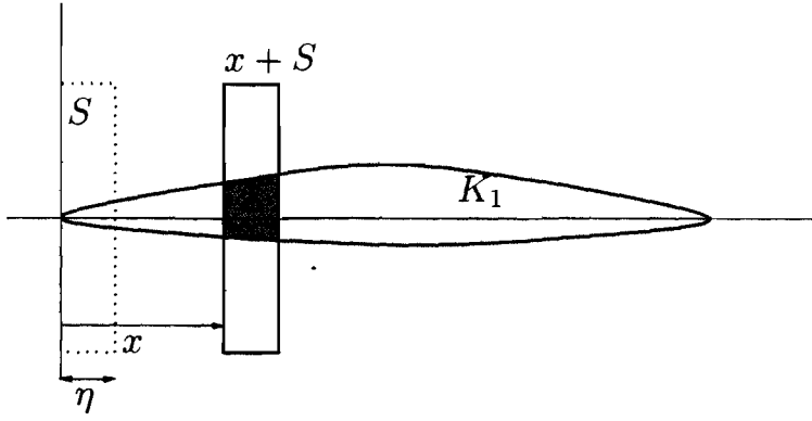
Figure 6.9: Slab S sweeping over K_1
