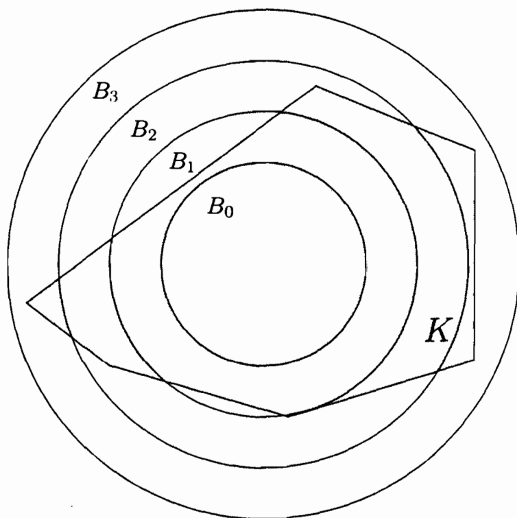
Figure 6.10: convex body K and the concentric balls
