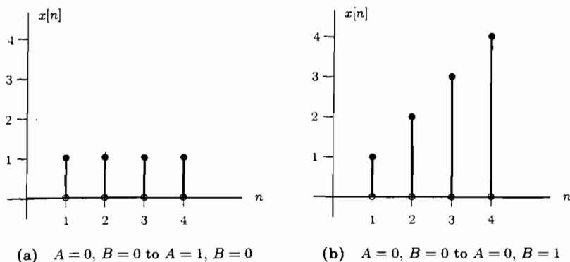
Figure 3.5 Sensitivity of observations to parameter changes—no noise
