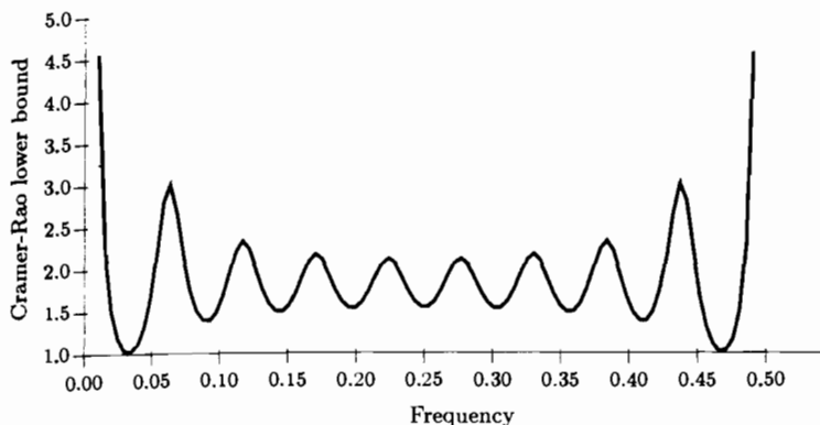
Figure 3.3 Cramer-Rao lower bound for sinusoidal frequency estimation
