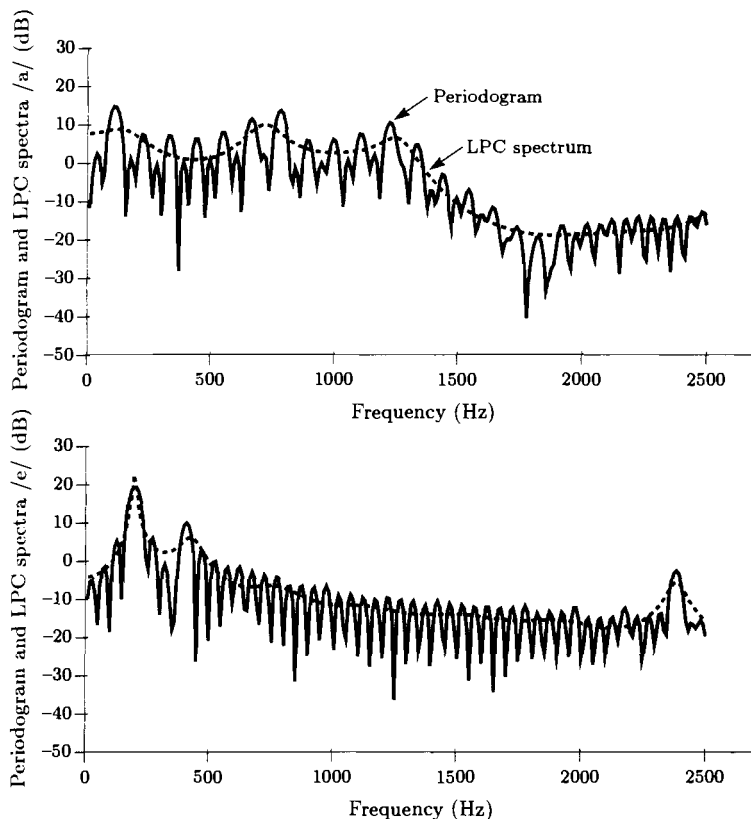
Figure 1.4 LPC spectral modeling
