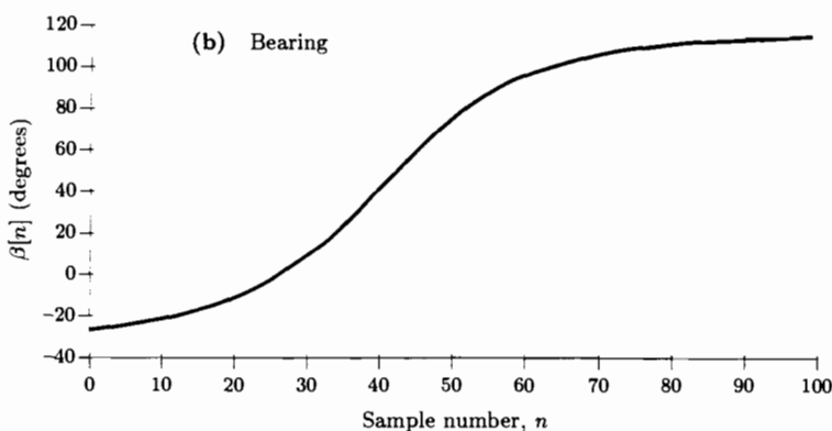
Figure 13.23 Range and bearing of true vehicle track
