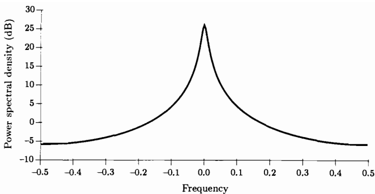
Figure 11.9 Power spectral density of AR(1) process
