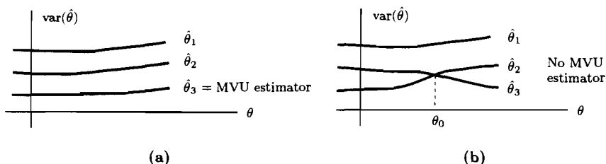
Figure 2.3 Possible dependence of estimator variance with \theta
