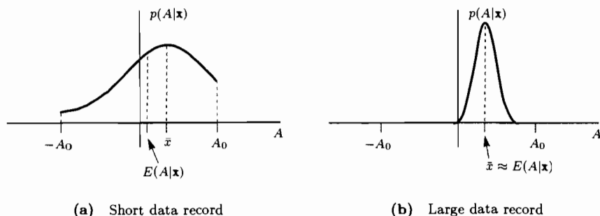
Figure 10.4 Effect of increasing data record on posterior PDF
