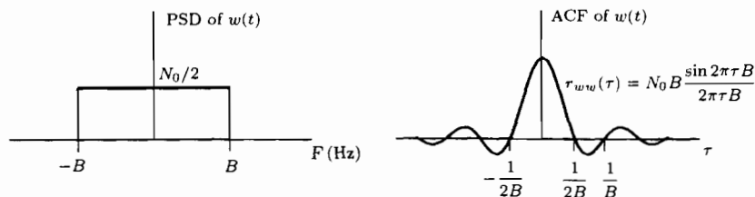
Figure 3.7 Properties of Gaussian observation noise
