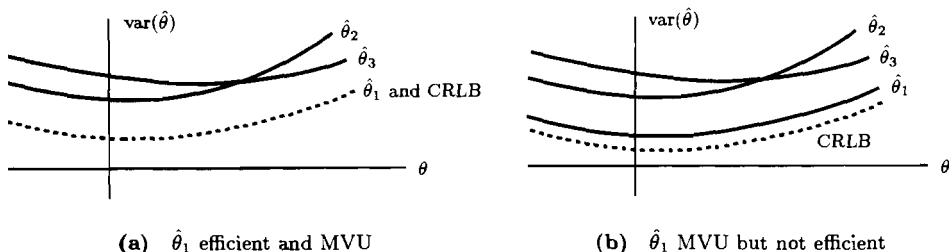
Figure 3.2 Efficiency vs. minimum variance
