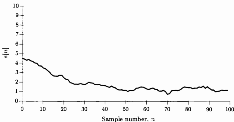
Figure 13.2 Typical realization of first order Gauss-Markov process
