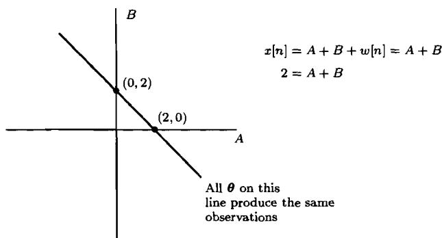
Figure 4.1 Nonidentifiability of linear model parameters
