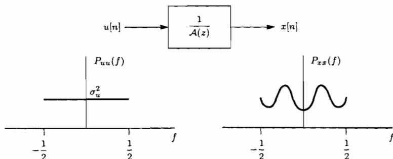
Figure 3.9 Autoregressive model
