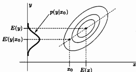
Figure 10.6 Contours of constant density for bivariate Gaussian PDF
