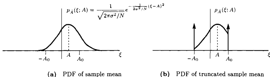
Figure 10.1 Improvement of estimator via prior knowledge
