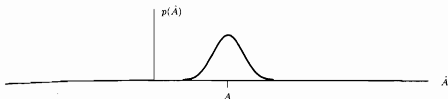
Figure 2.1 Probability density function for sample mean estimator
