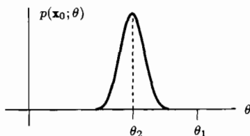
Figure 7.1 Rationale for maximum likelihood estimator
