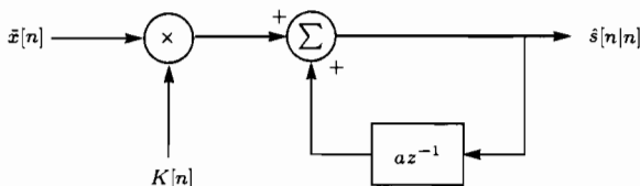
Figure 13.8 Innovation-driven Kalman filter
