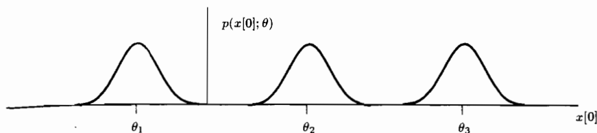
Figure 1.5 Dependence of PDF on unknown parameter
