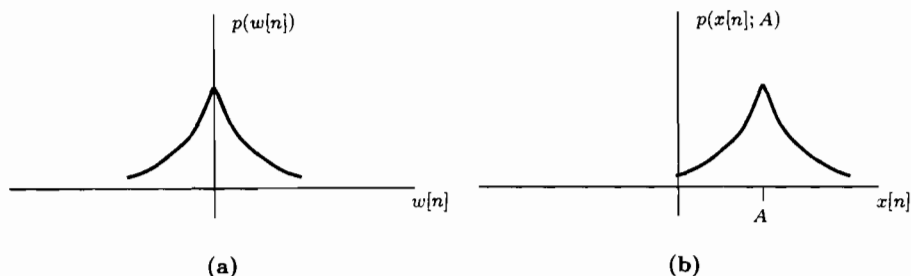
Figure 7.6 Non-Gaussian PDF for Example 7.7
