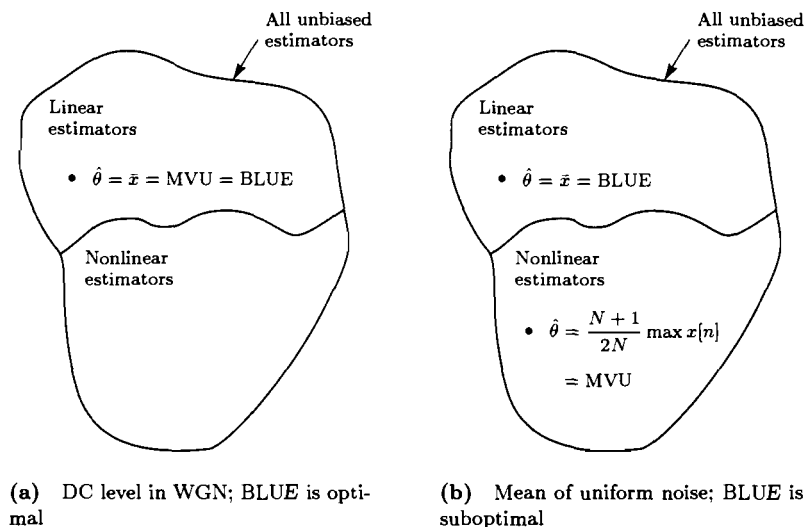
Figure 6.1 Optimality of BLUE
