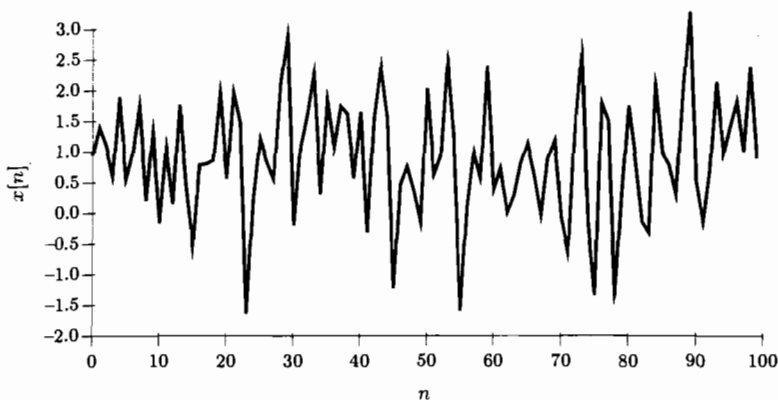
Figure 1.7 Realization of DC level in noise
