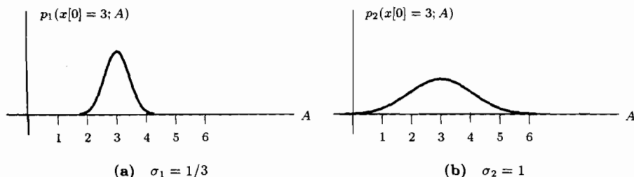
Figure 3.1 PDF dependence on unknown parameter
