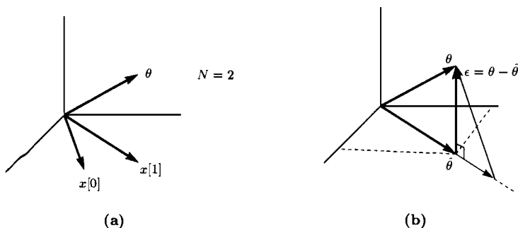
Figure 12.3 Orthogonality principle for LMMSE estimation
