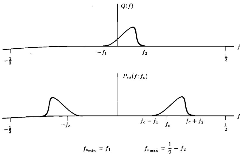
Figure 3.6 Signal PSD for center frequency estimation
