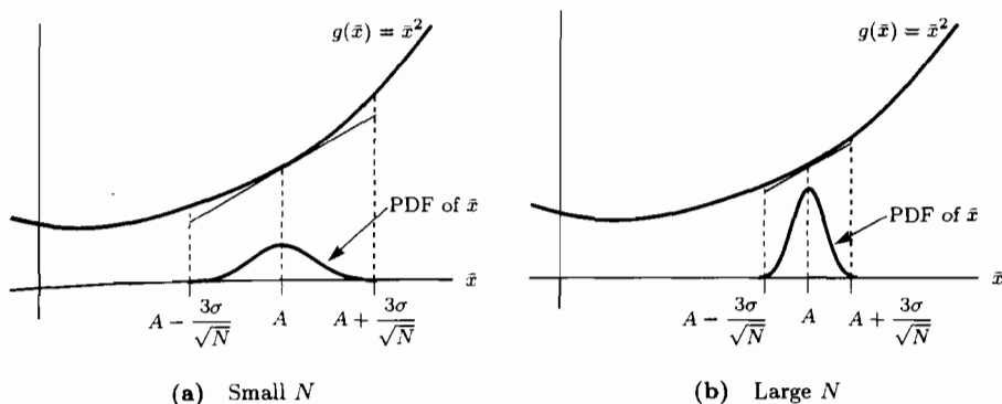
Figure 3.4 Statistical linearity of nonlinear transformations
