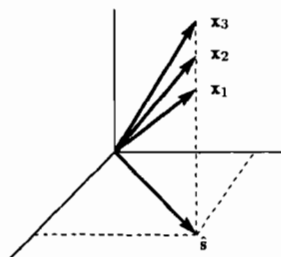
Figure 8.4 Vectors with same projection onto subspace
