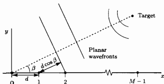
Figure 3.8 Geometry of array for bearing estimation
