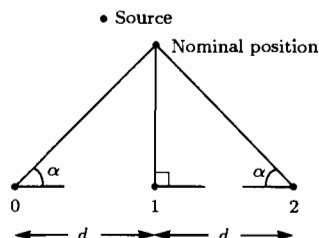
Figure 6.4 Example of source localization geometry for line array with minimum number of antennas
