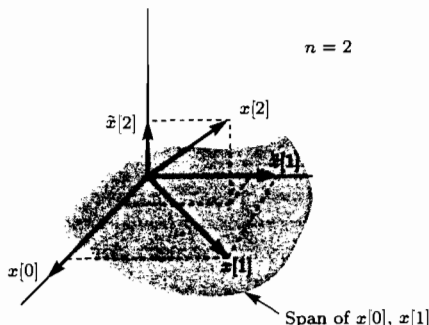
Figure 13.9 Orthogonality (uncorrelated property) of innovation sequence \tilde{x}(n)
