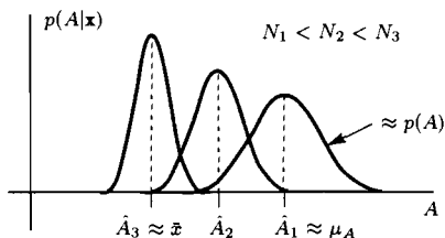
Figure 10.5 Effect of increasing data record length on posterior PDF
