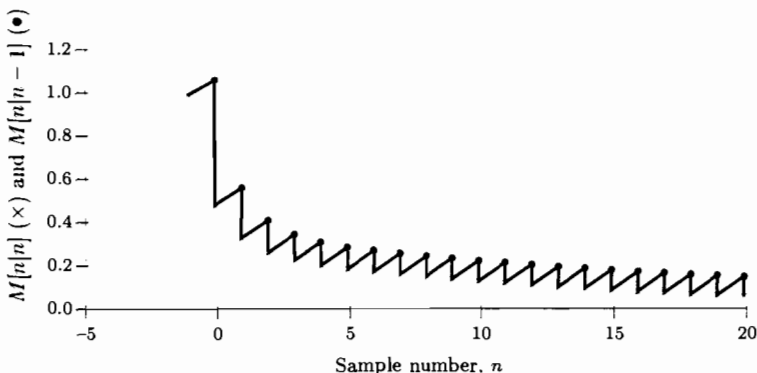
Figure 13.7 Prediction and correction minimum MSE
