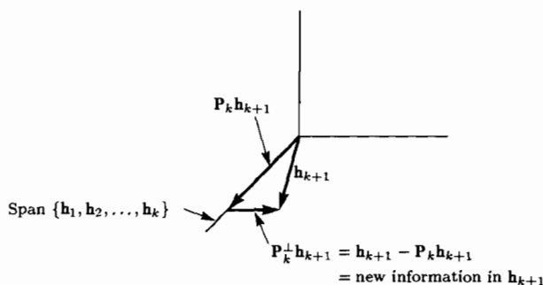
Figure 8.8 Near collinearity of columns of observation matrix
