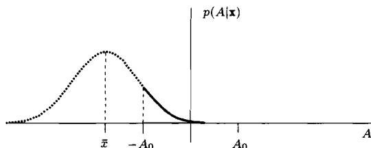
(c) \bar{x} < -A_0
