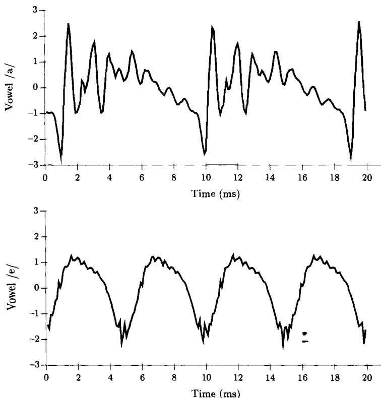
Figure 1.3 Examples of speech sounds
