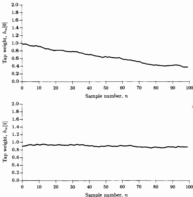
Figure 13.16 Realization of TDL coefficients
