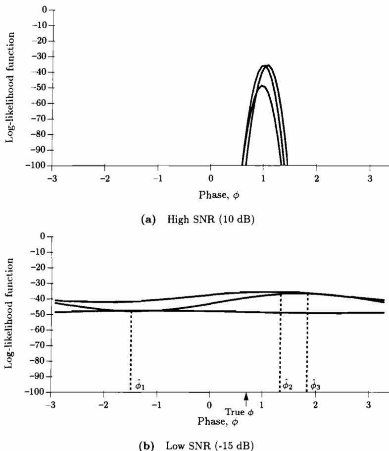
Figure 7.5 Typical realizations of log-likelihood function for phase
