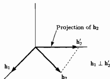
Figure 8.7 Gram-Schmidt orthogonalization
