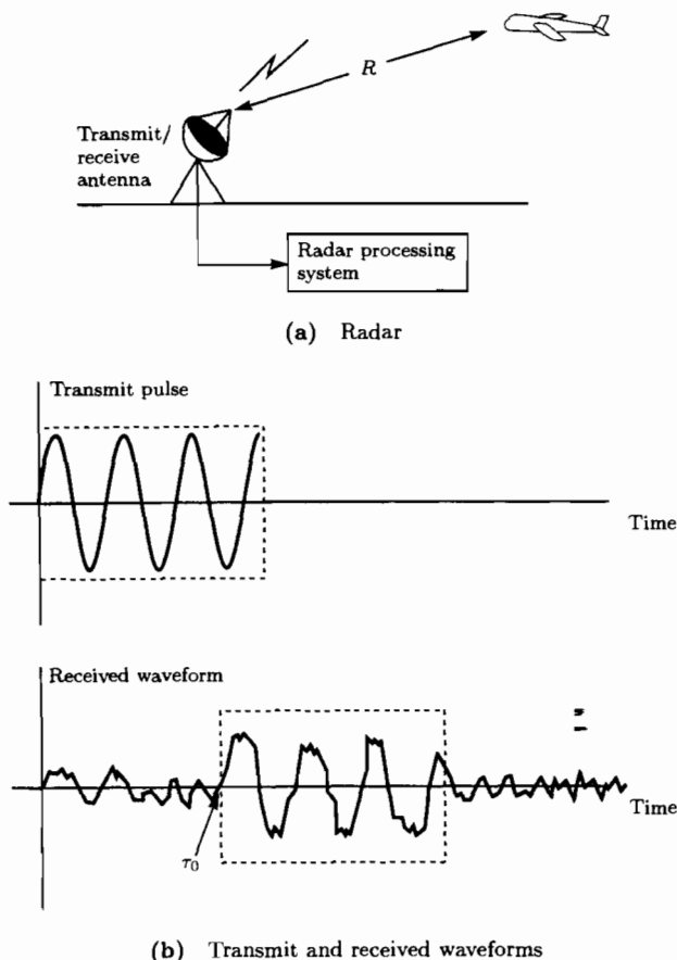
Figure 1.1 Radar system
