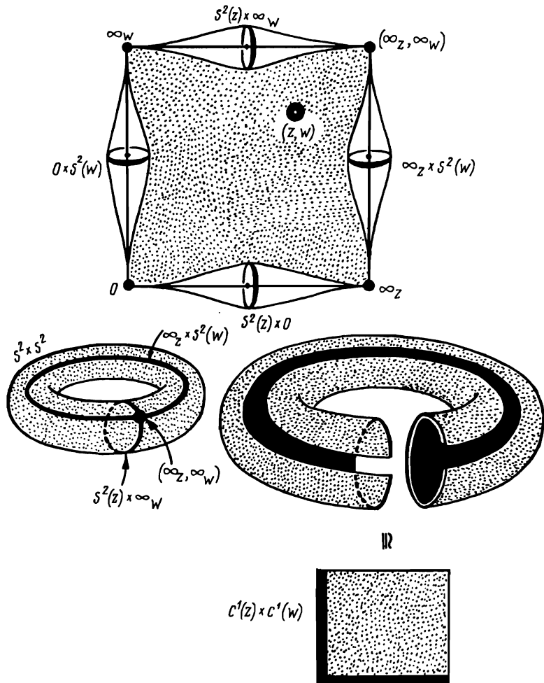
Рис. 120. (S^2 \times S^2) \setminus [(S^2(z) \times \infty_w) \cup (\infty_z \times S^2(w))] \cong \mathbb{C}^2(z, w)
