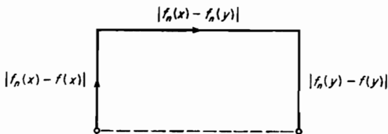
FIGURE I.7 The \epsilon/3 argument.
