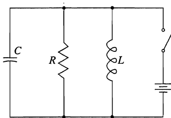
FIGURE 15.13 Ringing circuit.
