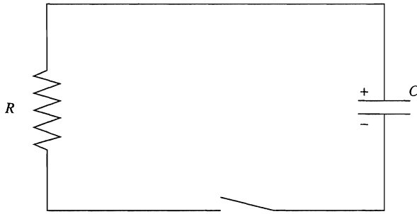
FIGURE 8.1 RC circuit.
