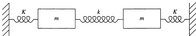
FIGURE 3.8 Oscillator.
