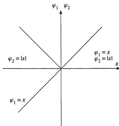
FIGURE 8.3 x and |x| .
