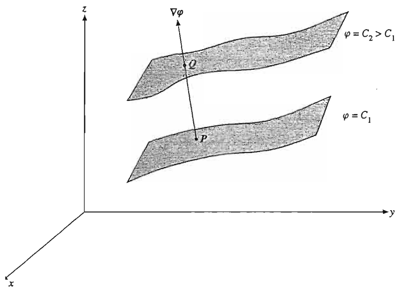
FIGURE 1.20 Gradient.
