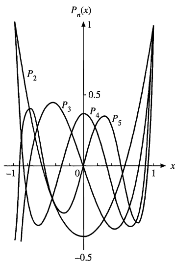
FIGURE 12.2 Legendre polynomials P_2(x) , P_3(x) , P_4(x) , and P_5(x) .
