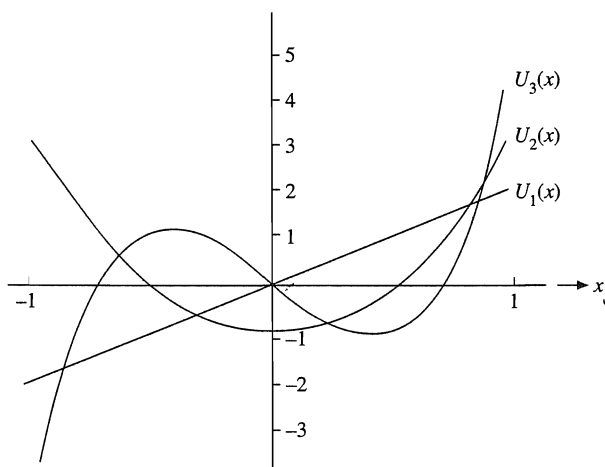
FIGURE 13.6 Chebyshev polynomials U_n(x) .
