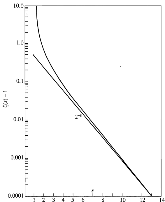
FIGURE 5.11 Riemann zeta function, \zeta(s) - 1 vs s .
