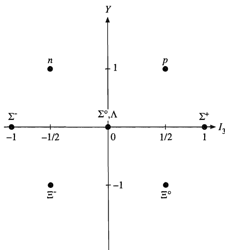
FIGURE 4.3 Baryon octet weight diagram for SU(3) .
