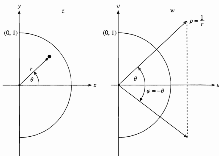
FIGURE 6.18 Inversion.
