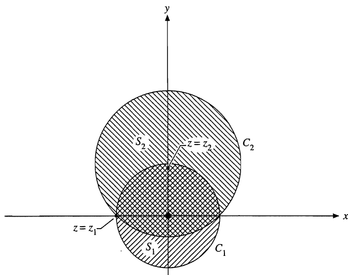
FIGURE 6.14 Analytic continuation.
