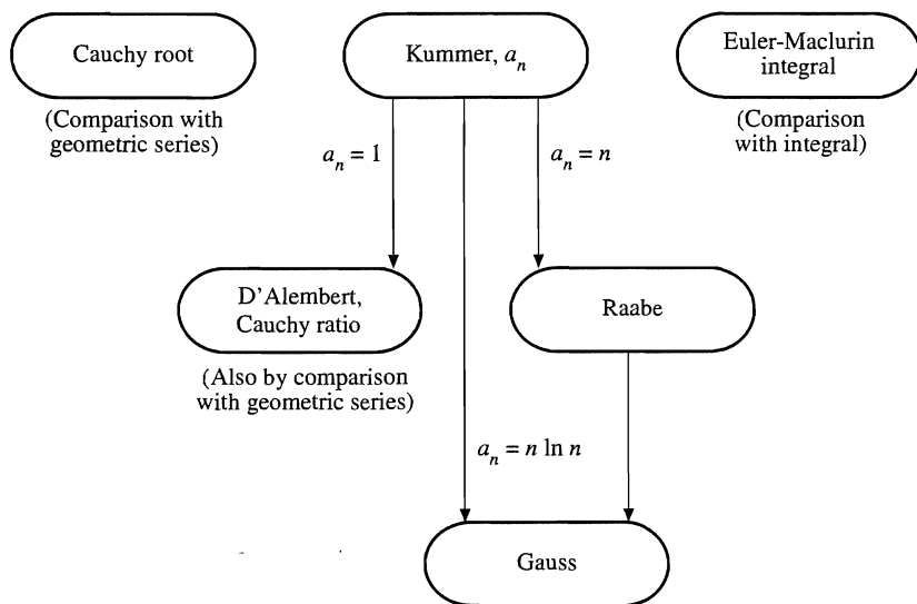
FIGURE 5.1 Comparison tests.
