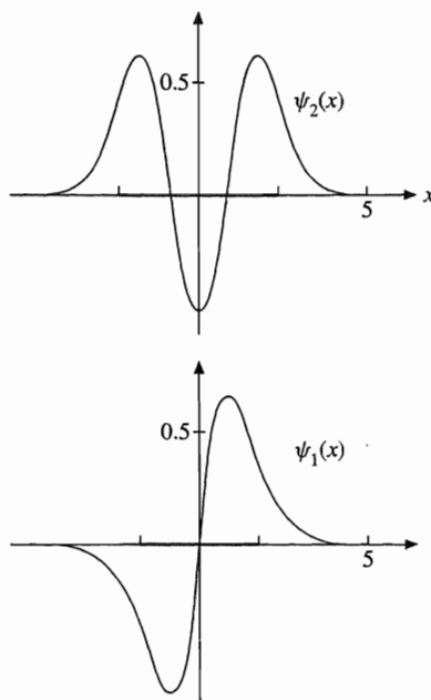
FIGURE 13.2 Quantum mechanical oscillator wavefunctions—the heavy bar on the x -axis indicates the allowed range of the classical oscillator with the same total energy.
