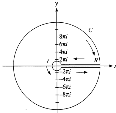
FIGURE 7.11 Contour of integration for Bernoulli numbers.
