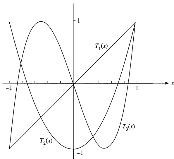
FIGURE 13.5 Chebyshev polynomials T_n(x) .
