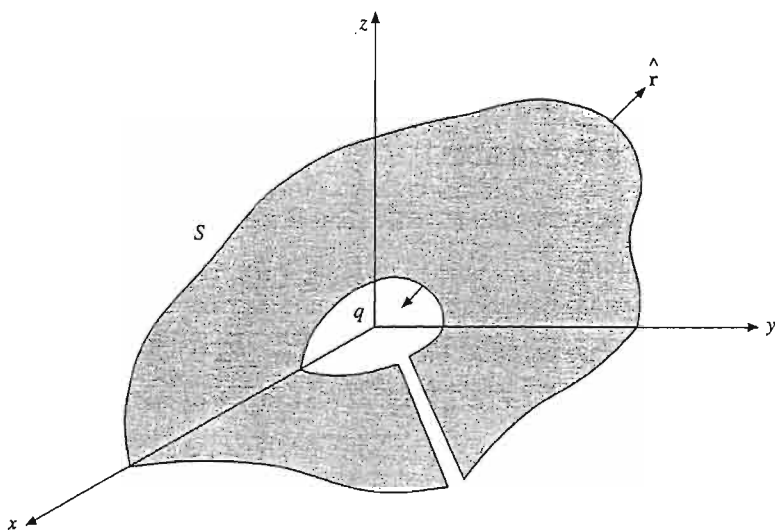
FIGURE 1.36 Exclusion of the origin.
