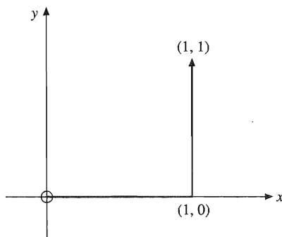
FIGURE 1.25 A path of integration.
