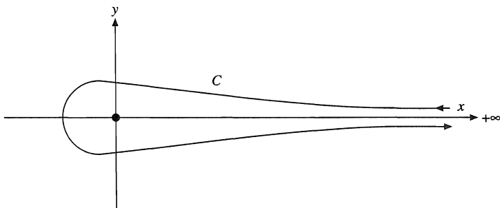
FIGURE 10.3 Factorial function contour.
