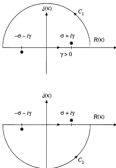
FIGURE 8.5 Possible Green's function contours of integration.
