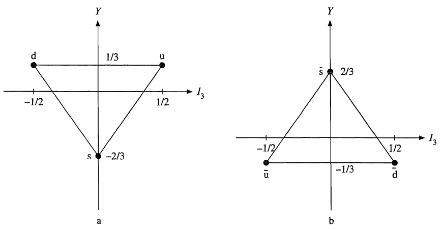
FIGURE 4.5 (a) Fundamental representation of SU(3), the weight diagram for the u , d , s quarks; (b) weight diagram for the antiquarks \bar{u} , \bar{d} , \bar{s} .
