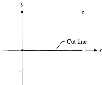
FIGURE 6.21 A cut line.
