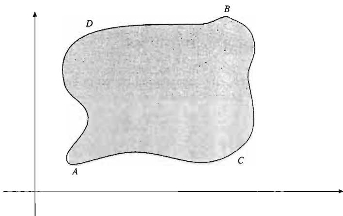
FIGURE 1.32 Possible paths for doing work.
