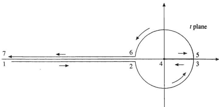
FIGURE 6.23 Bessel function integration contour.
