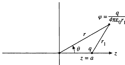
FIGURE 12.1 Electrostatic potential. Charge q displaced from origin.
