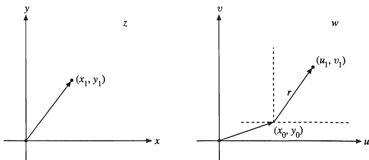
FIGURE 6.16 Translation.
