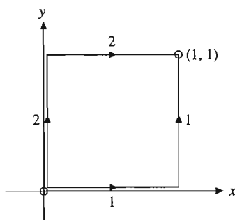
FIGURE 6.10 Contour for Exercise 6.3.3.
