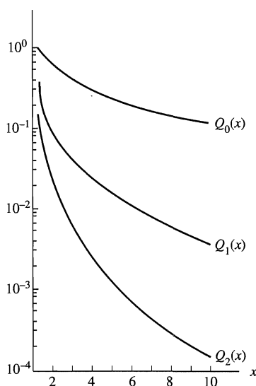
FIGURE 12.17 Second Legendre function Q_n(x) , x > 1 .
