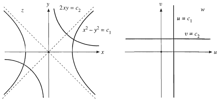
FIGURE 6.20 Mapping—hyperbolic coordinates.
