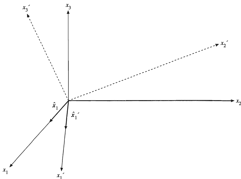
FIGURE 3.1 Cartesian coordinate systems.
