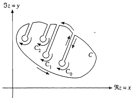
FIGURE 7.2 Excluding isolated singularities.
