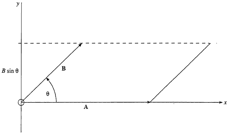
FIGURE 1.13 Parallelogram representation of the vector product.
