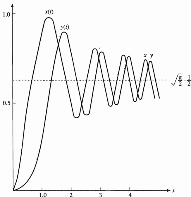
FIGURE 11.15 Fresnel integrals.
