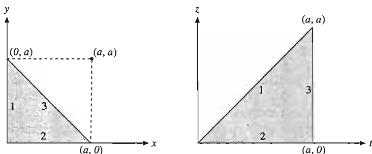
FIGURE 15.15 Change of variables, (a) xy -plane (b) zt -plane.
