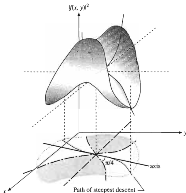
FIGURE 7.19 A saddle point.
