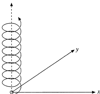
FIGURE 6.22 This is the Riemann surface for \ln z , which is a multivalued function.
