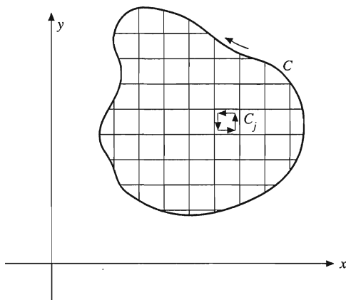
FIGURE 6.7 Cauchy-Goursat contours.
