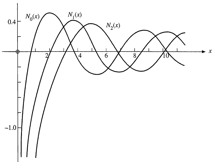
FIGURE 11.5 Neumann functions N_0(x) , N_1(x) , and N_2(x) .
