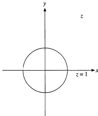
FIGURE 13.3 Laguerre function contour.
