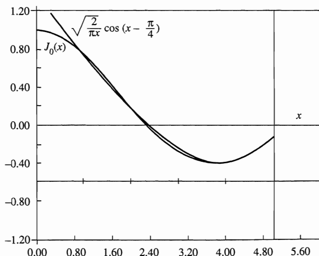
FIGURE 11.11 Asymptotic approximation of J_0(x) .
