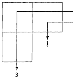
FIGURE 4.9 Illustration of (a) N and (b) D in Eq. (4.125) for the octet Young tableau of SU(3) .
