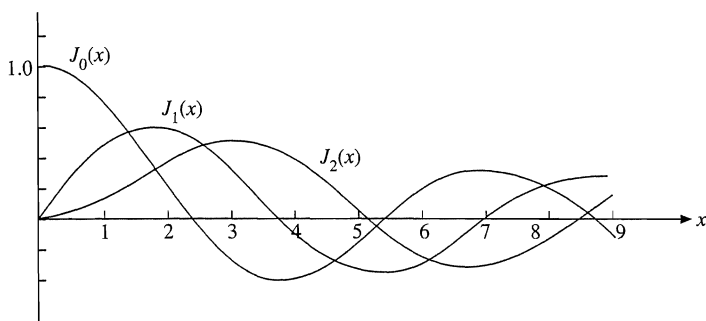
FIGURE 11.1 Bessel functions, J_0(x) , J_1(x) , and J_2(x) .
