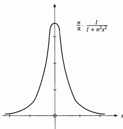
FIGURE 1.39 \delta -sequence function.
