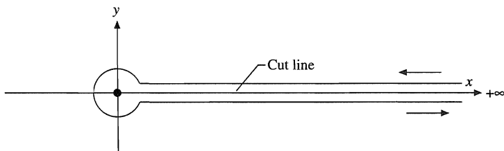
FIGURE 10.4 The contour of Fig. 10.3 deformed.
