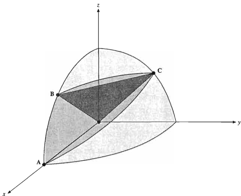
FIGURE 1.14 Spherical triangle.
