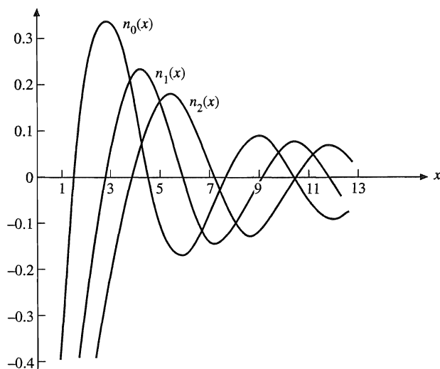
FIGURE 11.14 Spherical Neumann functions.
