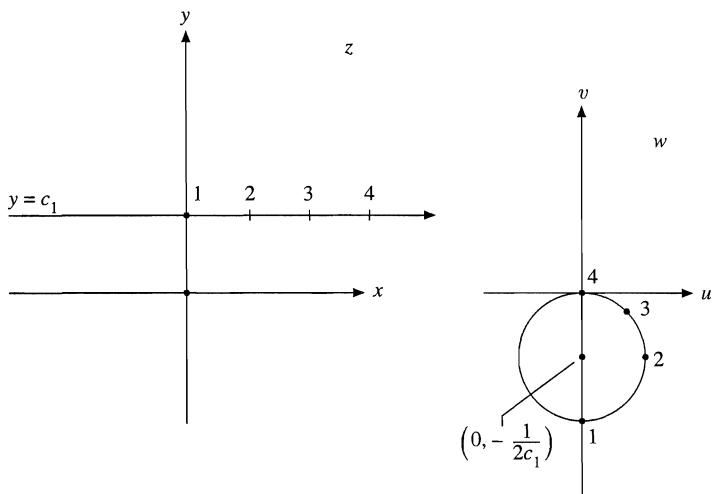
FIGURE 6.19 Inversion, line \leftrightarrow circle.
