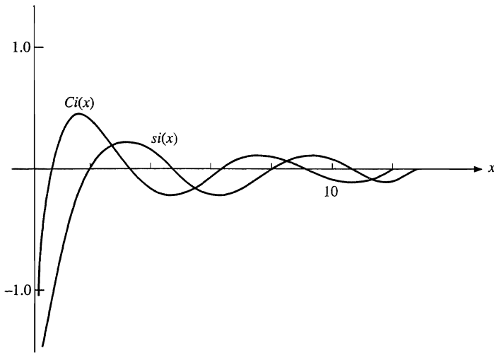
FIGURE 10.8 Sine and cosine integrals.
