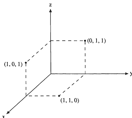
FIGURE 3.6 Mass sites for inertia tensor.
