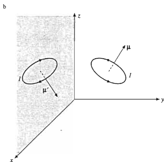
FIGURE 2.10 (a) Mirror in xz -plane; (b) Mirror in xz -plane.
