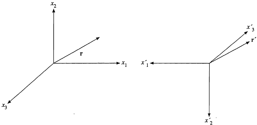
FIGURE 2.8 Inversion of Cartesian coordinates — polar vector.
