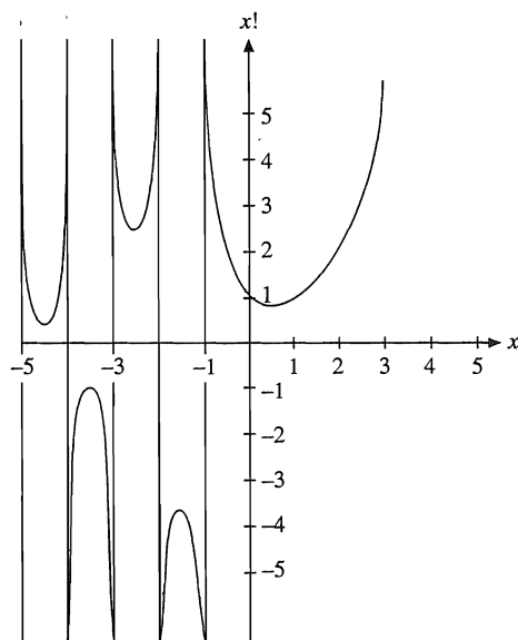
FIGURE 10.1 The factorial function—extension to negative arguments.
