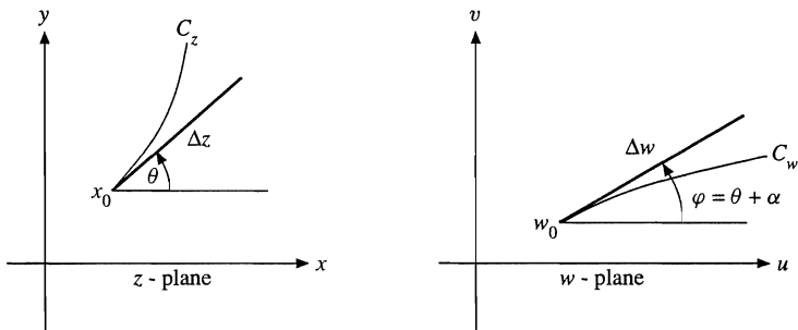
FIGURE 6.24 Conformal mapping—preservation of angles.
