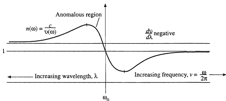
FIGURE 15.18 Optical dispersion.
