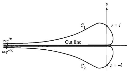
FIGURE 7.20 Hankel function contours.
