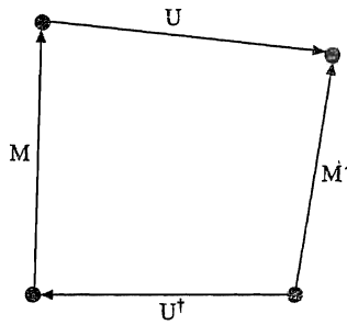
FIGURE 4.2 Illustration of M' = U M U^\dagger in Eq. (4.43).
