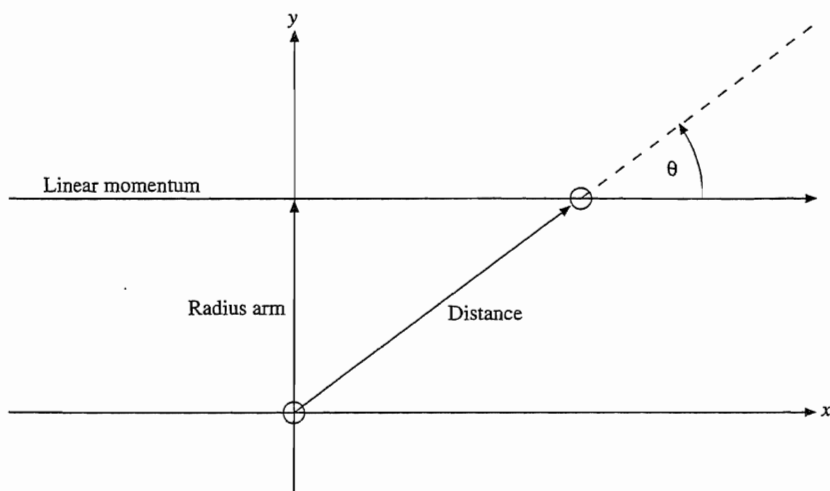
FIGURE 1.12 Angular momentum.
