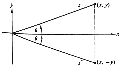
FIGURE 6.3 Complex conjugate points.
