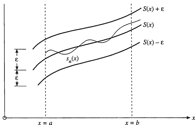
FIGURE 5.7 Uniform convergence.
