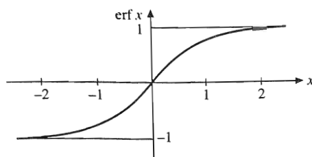
FIGURE 10.9 Error function \operatorname{erf} x .
