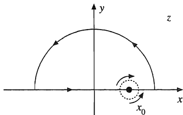
FIGURE 7.4 Closing the contour with an infinite radius semicircle.
