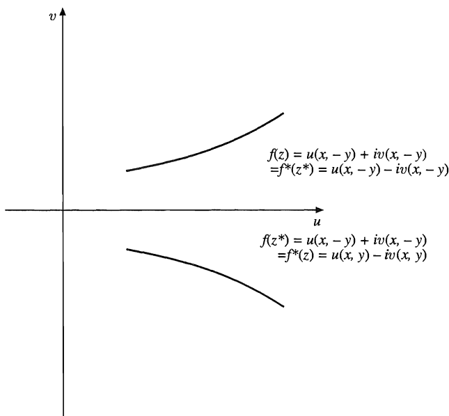
FIGURE 6.13 Schwarz reflection.
