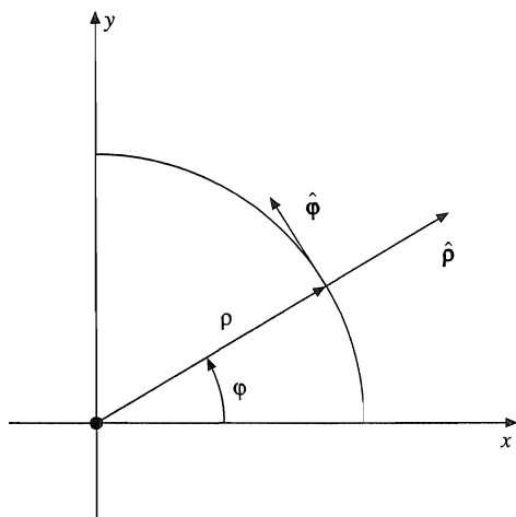
FIGURE 2.5 Plane polar coordinates.
