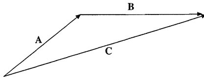
FIGURE 1.1 Triangle law of vector addition.
