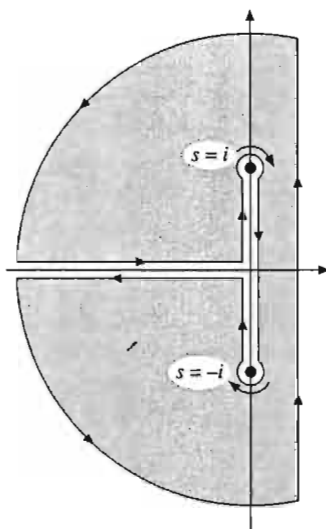
FIGURE 15.20 A possible contour for the inversion of J_0(t) .
