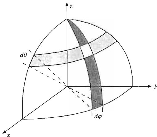
FIGURE 2.6 Spherical polar coordinate area elements.
