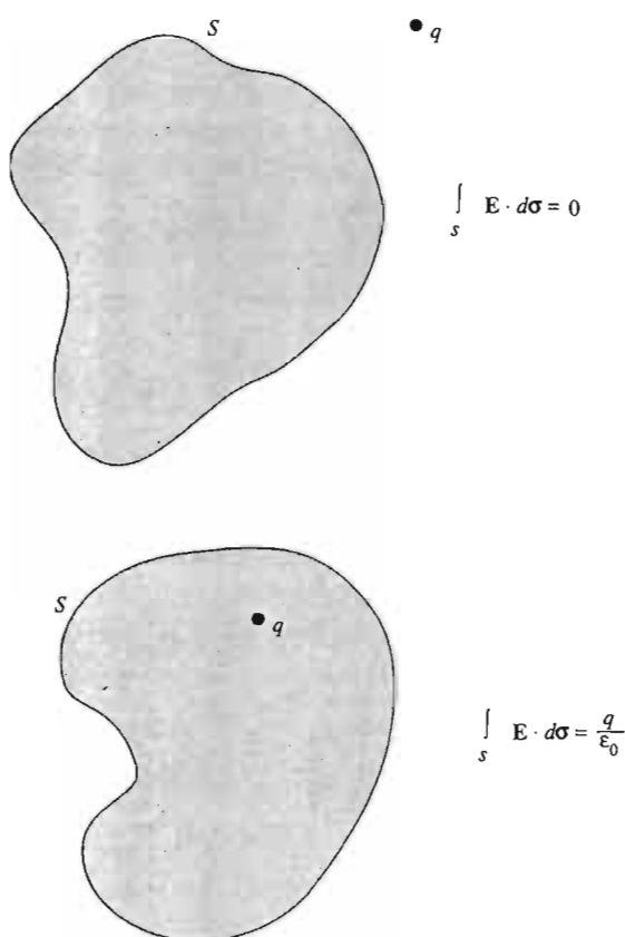
FIGURE 1.35 Gauss's law.
