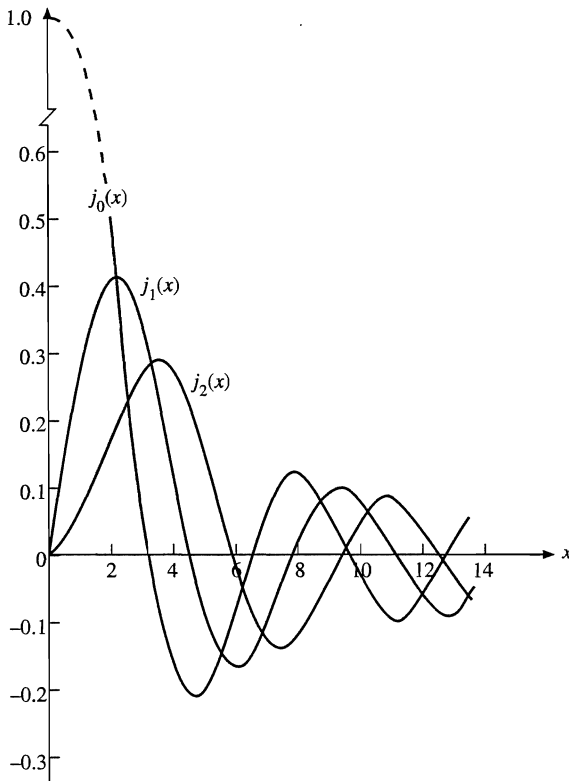
FIGURE 11.13 Spherical Bessel functions.
