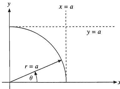
FIGURE 10.6 Transformation from Cartesian to polar coordinates.
