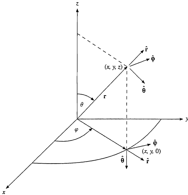
FIGURE 2.7 Spherical polar coordinates.
