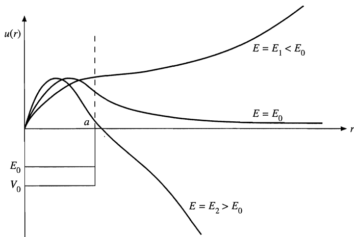
FIGURE 9.1 A deuteron eigenfunction.
