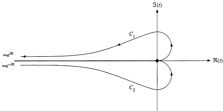
FIGURE 11.8 Hankel function contours.
