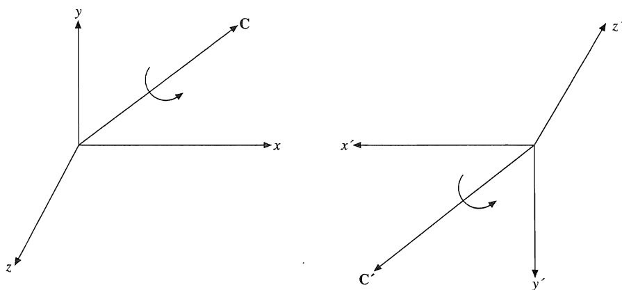
FIGURE 2.9 Inversion of Cartesian coordinates — axial vector.
