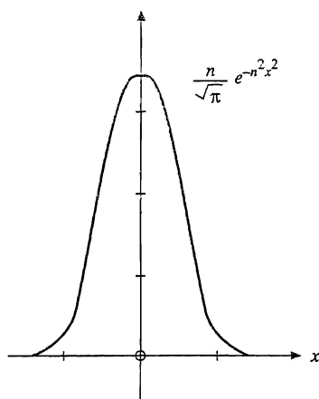
FIGURE 1.38 \delta -sequence function.
