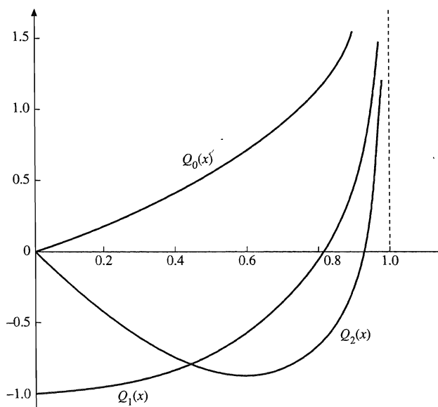
FIGURE 12.16 Second Legendre function Q_n(x) , 0 \leq x < 1 .
