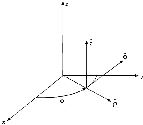
FIGURE 2.4 Circular cylindrical coordinate unit vectors.
