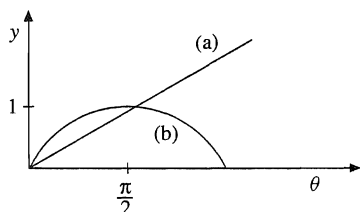
FIGURE 7.7 (a) y = (2/\pi)\theta , (b) y = \sin \theta .
