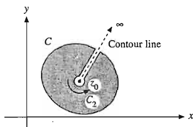
FIGURE 6.11 Exclusion of a singular point.
