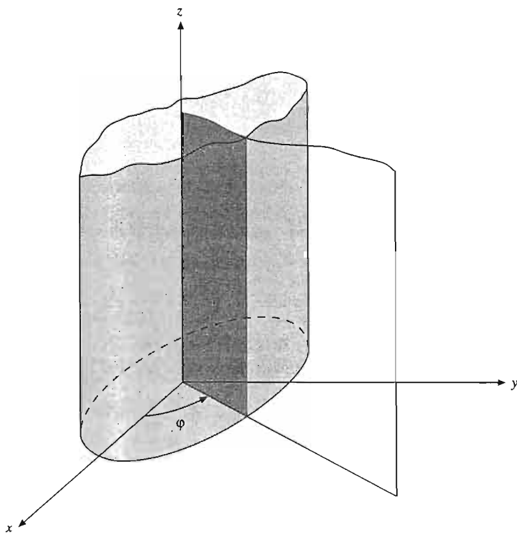
FIGURE 2.3 Circular cylindrical coordinates.
