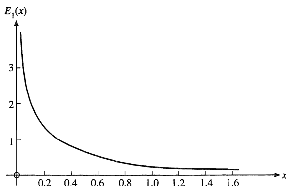
FIGURE 10.7 The exponential integral E_1(x) = -Ei(-x) .
