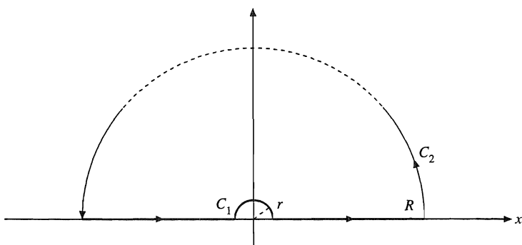
FIGURE 7.8 Singularity on contour
