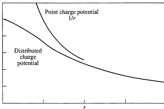
FIGURE 10.10 Distributed charge potential produced by a 1s hydrogen electron; see Exercise 10.5.14.
