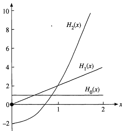
FIGURE 13.1 Hermite polynomials.
