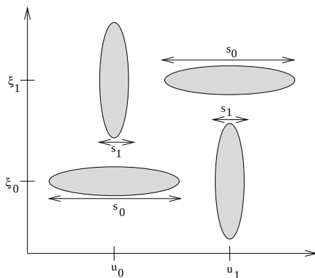
Figure 9.9: Time-frequency energy distribution of the four elementary atoms in (9.69).
