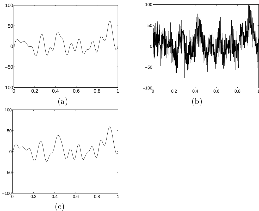
Figure 10.1: (a): Realization of a Gaussian process F . (b): Noisy signal obtained by adding a Gaussian white noise (SNR = -0.48 db). (c): Wiener estimation \tilde{F} (SNR = 15.2 db).
