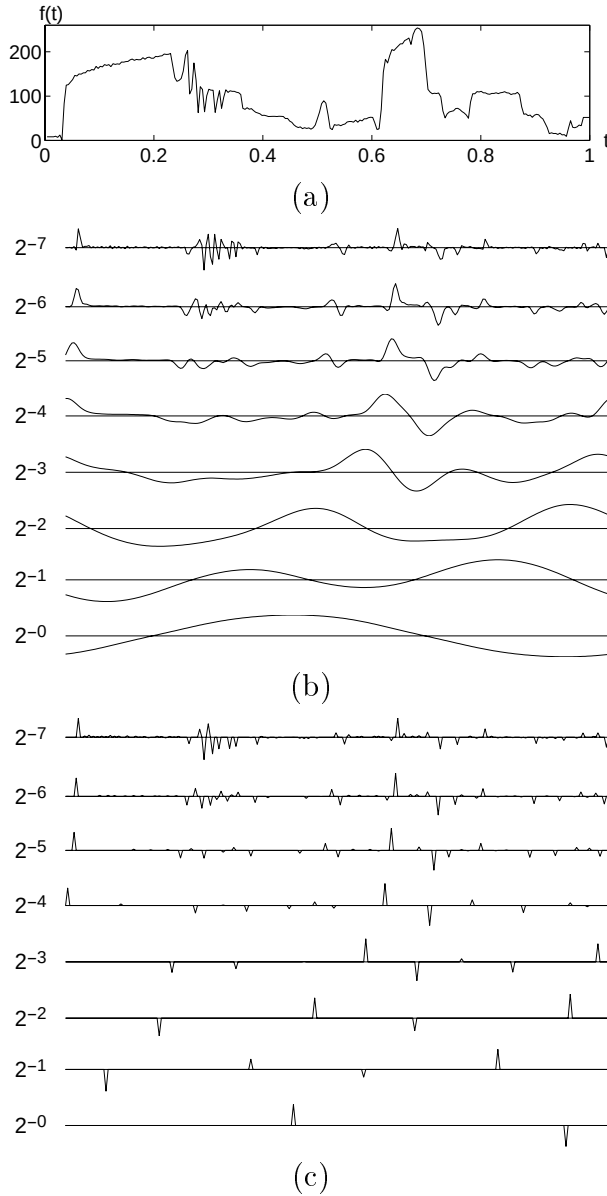
Figure 6.7: (a): Intensity variation along one row of the Lena image. (b): Dyadic wavelet transform computed at all scales 2N^{-1} \leq 2^j \leq 1 , with the quadratic spline wavelet \psi = -\theta' shown in Figure 5.6. (c): Modulus maxima of the dyadic wavelet transform.
