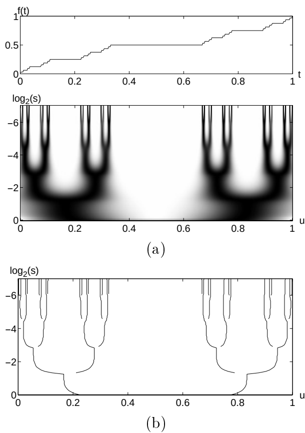
Figure 6.16: Devil's staircase calculated from a Cantor measure with equal weights p_1 = p_2 = 0.5 . (a): Wavelet transform Wf(u, s) computed with \psi = -\theta' , where \theta is Gaussian. (b): Wavelet transform modulus maxima.
