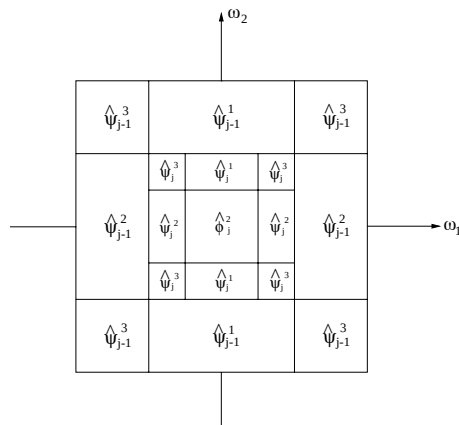
Figure 7.25: These dyadic rectangles indicate the regions where the energy of \hat{\psi}_{j,n}^k is mostly concentrated, for 1 \leq k \leq 3 . Image approximations at the scale 2^j are restricted to the lower frequency square.
