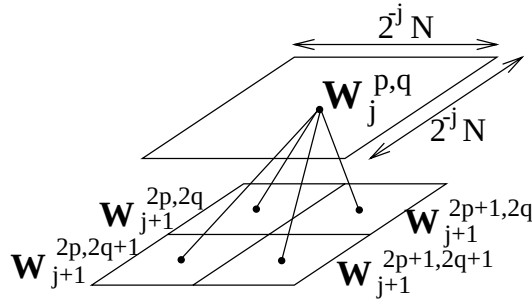
Figure 8.21: Functions in \mathbf{W}_j^{p,q} have a support located in a square region of the image. It is divided into four subspaces that cover smaller squares in the image.
