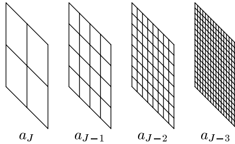
Figure 11.20: The pixels of an image approximation a_j correspond to averages of the image intensity over blocks of width proportional to N 2^j .
