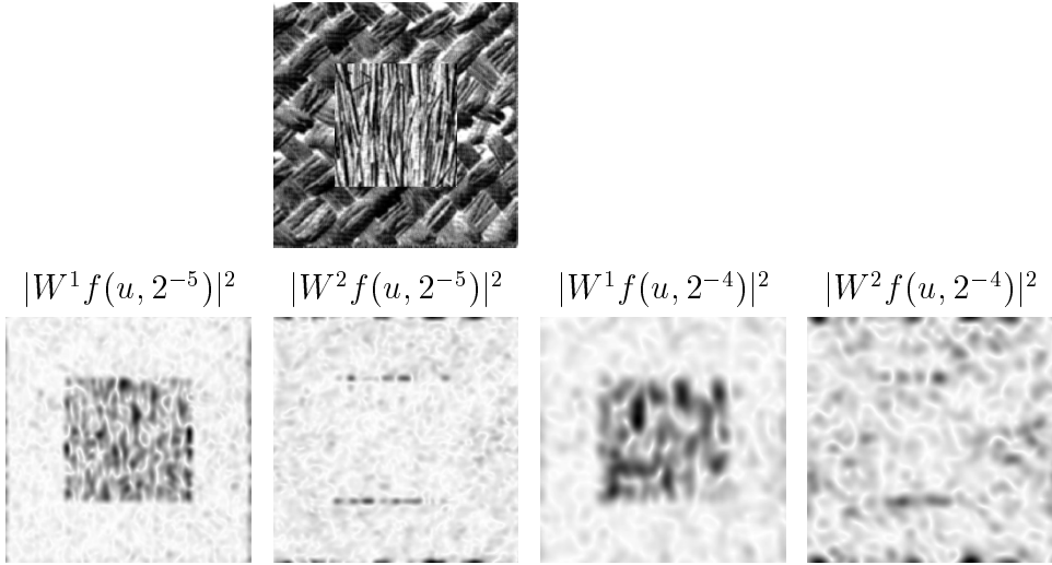
Figure 5.9: Gabor wavelet transform |W^k f(u, 2^j)|^2 of a texture patch, at the scales 2^{-4} and 2^{-5} , along two orientations \alpha_k respectively equal to 0 and \pi/2 for k = 1 and k = 2 . The darker a pixel, the larger the wavelet coefficient amplitude.
