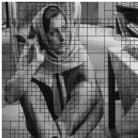
Figure 9.11: The grid shows the approximate support of square overlapping windows in the best local cosine basis, computed with an \mathbf{l}^1 cost.
