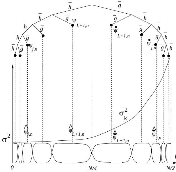
Figure 10.11: Wavelets and mirror wavelets are computed with a wavelet packet filter bank tree, where each branch corresponds to a convolution with a filter \bar{h} or \bar{g} followed by a subsampling. The graphs of the discrete Fourier transforms |\hat{\psi}_{j,n}[k]| and |\hat{\psi}_{j,n}[k]| are shown below the tree. The variance \sigma_k^2 of the noise has a hyperbolic growth but varies by a bounded factor on the frequency support of each mirror wavelet.
