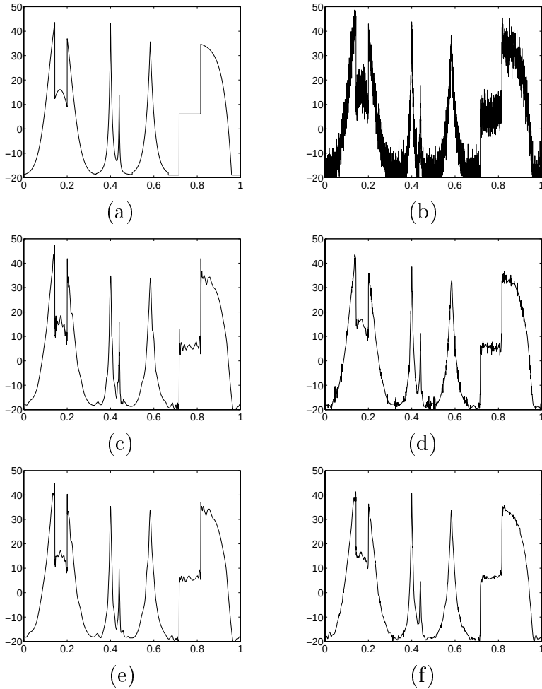
Figure 10.5: (a): Original signal. (b): Noisy signal (SNR = 13.1 db). (c): Estimation by a hard thresholding in a wavelet basis (Symmlet 4), with T = \tilde{\sigma}\sqrt{2\log_e N} (SNR = 23.3 db). (d): Soft thresholding calculated with SURE thresholds T_j adapted to each scale 2^j (SNR = 24.5 db). (e): Translation invariant hard thresholding with T = \tilde{\sigma}\sqrt{2\log_e N} (SNR = 25.7 db). (f): Translation invariant soft thresholding with SURE thresholds (SNR = 25.6 db).
