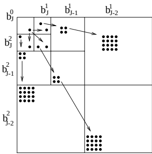
Figure 11.18: At the coarsest scale 2^J , the children of each pixel in b_j^0 are the three pixels of the same position in b_j^1 , b_j^2 and b_j^3 . At all other scales, in each direction l , quad-trees are constructed by relating a pixel of b_j^l to its four children in b_{j-1}^l .
