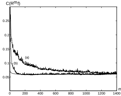
Figure 10.16: Decay of the correlation \mathcal{C}(R^m f) as a function of the number of iterations m , for two signals decomposed in a Gabor dictionary. (a): f is the recording of “greasy” shown in Figure 10.17(a). (b): f is the noisy “greasy” signal shown in Figure 10.17(b).
