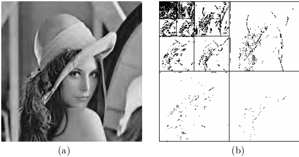
Figure 9.4: (a): Non-linear approximation f_M of a Lena image f of N^2 = 256^2 pixels, with M = N^2/16 wavelet coefficients: \|f - f_M\|/\|f\| = 0.011 . Compare with the linear approximation of Figure 9.2(b). (b): The positions of the largest M wavelet coefficients are shown in black.
