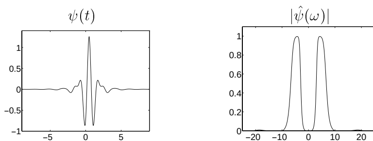
Figure 7.5: Battle-Lemarié cubic spline wavelet \psi and its Fourier transform modulus.
