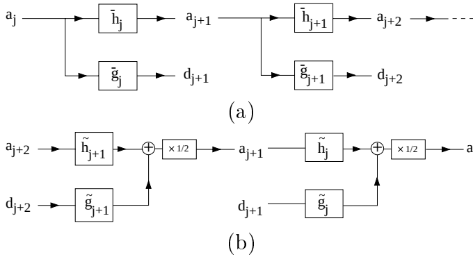
Figure 5.7: (a): The dyadic wavelet coefficients are computed by cascading convolutions with dilated filters \bar{h}_j and \bar{g}_j . (b): The original signal is reconstructed through convolutions with \tilde{h}_j and \tilde{g}_j . A multiplication by 1/2 is necessary to recover the next finer scale signal a_j .
