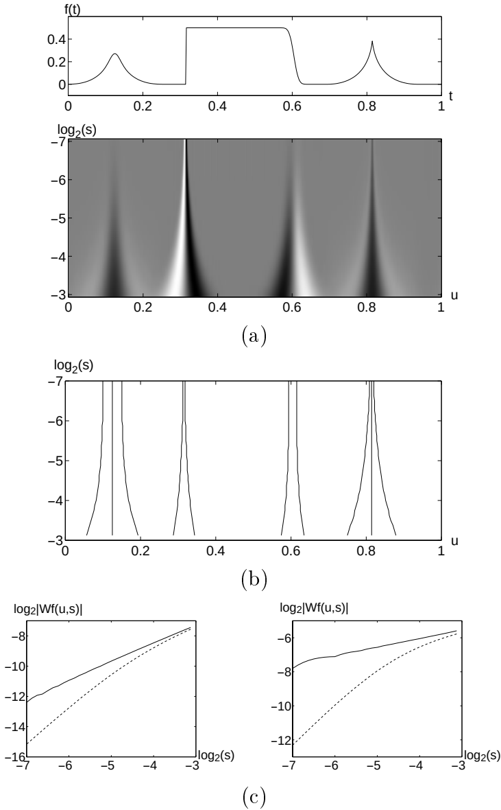
Figure 6.6: (a): Wavelet transform Wf(u, s) . (b): Modulus maxima of a wavelet transform computed \psi = \theta'' , where \theta is a Gaussian with variance \beta = 1 . (c): Decay of \log_2 |Wf(u, s)| along maxima curves. In the left figure, the solid and dotted lines correspond respectively to the maxima curves converging to t = 0.81 and t = 0.12 . In the right figure, they correspond respectively to the curves converging to t = 0.38 and t = 0.55 . The diffusion at t = 0.12 and t = 0.55 modifies the decay for s \leq \sigma = 2^{-5} .
