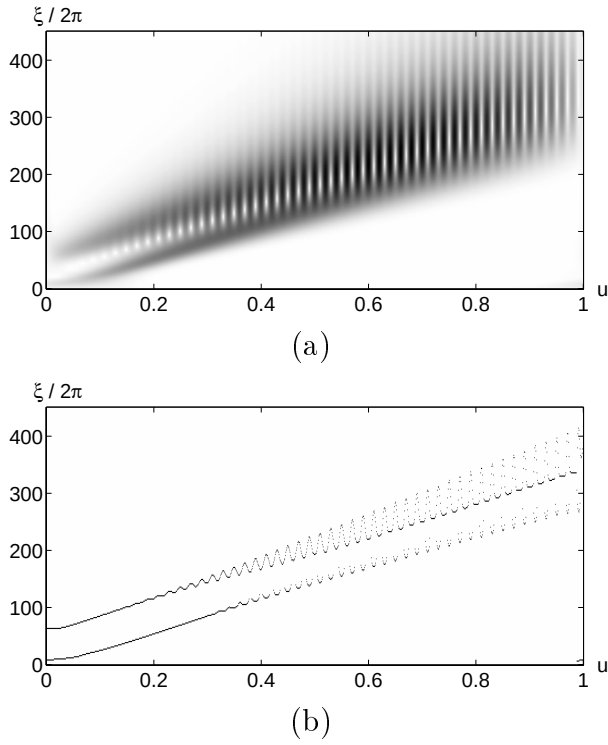
Figure 4.16: (a): Normalized scalogram \eta^{-1}\xi P_W f(u, \xi) of two parallel linear chirps shown in Figure 4.13. (b): Wavelet ridges.
