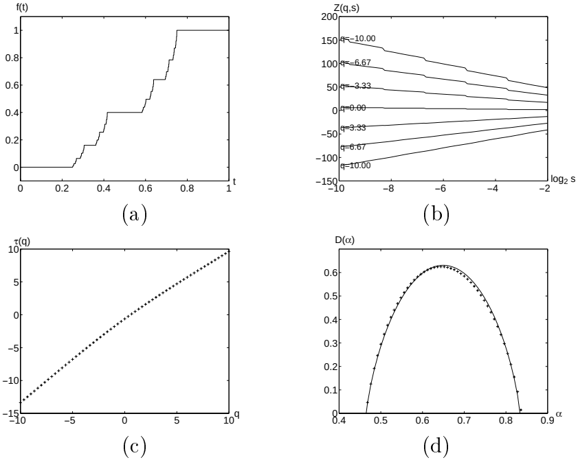
Figure 6.18: (a): Devil's staircase with p_1 = 0.4 and p_2 = 0.6 . (b): Partition function Z(q, s) for several values of q . (c): Scaling exponent \tau(q) . (d): The theoretical spectrum D(\alpha) is shown with a solid line. The + are the spectrum values calculated numerically with a Legendre transform of \tau(q) .
