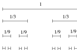
Figure 6.14: Three iterations of the Cantor subdivision of [0, 1] . The limit of an infinite number of subdivisions is a closed set in [0, 1] .
