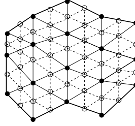
Figure 7.17: Black dots are the nodes of a triangulation grid \mathcal{G}_{j+1} of a polygon domain D . This grid is refined with a subdivision, which adds a complementary grid \mathcal{C}_{j+1} composed of all midpoints indicated with white circles. The finer grid is \mathcal{G}_j = \mathcal{G}_{j+1} \cup \mathcal{C}_{j+1} .
