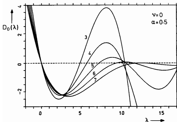
Fig. 12.14. The value of the determinant (9.119) for m=0 as a function of \lambda for various pump parameters a=3, \dots, 7 . The upper index \nu is zero and the scaling parameter \alpha is 0.5
