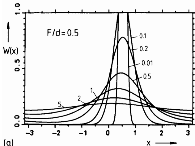
Fig. 11.9. The stationary distribution function W(x) for various temperatures \Theta/d and for F/d = 0.5 (a), F/d = 1 (b), F/d = 1.5 (c). In (c) the curve for \Theta/d = 0.01 practically agrees with the zero-temperature distribution (11.53)
