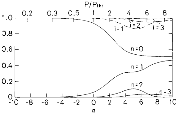
Fig. 12.8. The values \lambda_{1n} V_n^{(g)} \times g(a,0)/2 (solid line) for n = 0, 1, 2, 3 and the sum terms \sum_{n=0}^i \lambda_{1n} \times V_n^{(g)} g(a,0)/2 (dashed line) for i = 1, 2, 3 as a function of the pump parameter a and as a function of the power output P/P_{\text{thr}} , respectively
