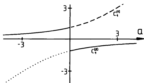
Fig. 9.1. Solution c_1^{(1)} (upper curve), solution c_1^{(2)} (lower curve) and the continued-fraction solution (9.43) (solid line) as a function of the parameter a
