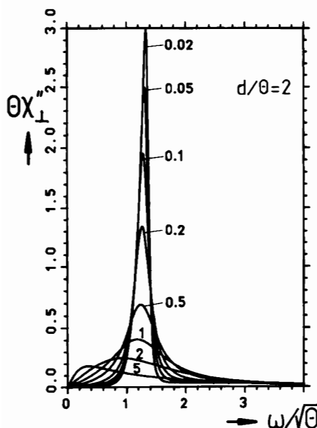
Fig. 11.38. Same as Fig. 11.36 b, but for d/\theta = 2
