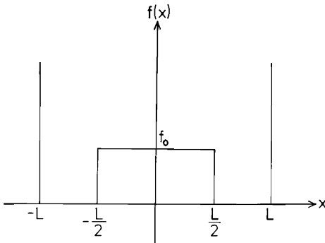
Fig. 5.3. Bistable potential model
