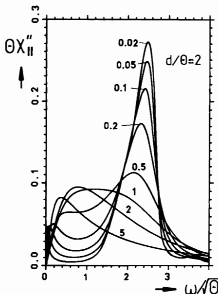
Fig. 11.39. Same as Fig. 11.37 b, but for d/\theta = 2
