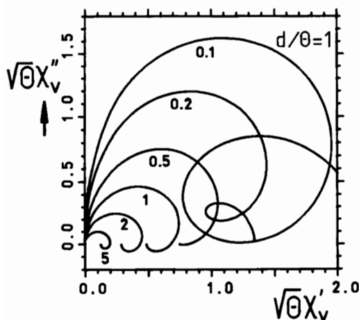
Fig. 11.33. The negative imaginary part times |\Theta| as a function of the real part of the susceptibilities for the parameters of Fig. 11.32. The frequency varies along the curve and is infinite at the origin
