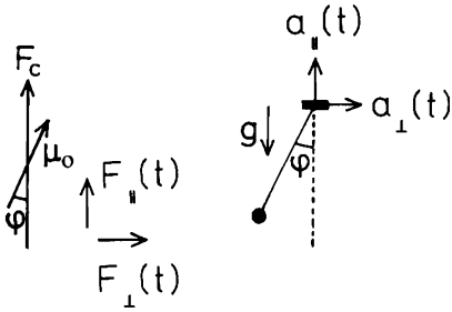
Fig. 11.6. Rotation of a dipole with moment \mu_0 in a constant field F_c and additional time-varying field parallel and perpendicular to F_c . The equation of motion is equivalent to that of a pendulum where the support is accelerated parallel and perpendicular to the gravitational force
