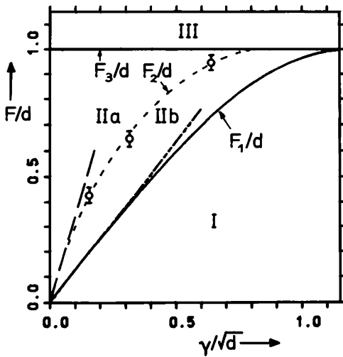
Fig. 11.26. The three critical forces F_1/d , F_2/d and F_3/d as a function of the friction constant \gamma/\sqrt{d} for the cosine potential (11.103). The straight lines --- and --- are the low-friction approximations F_1 = (4/\pi)\sqrt{d}\gamma and F_2 = F_{02}\gamma , with F_{02} given by (11.196). The circles indicate extrapolations for \Theta \rightarrow 0 of the critical force F_2/d calculated with the matrix continued-fraction method. For the meaning of Regions I, IIa, IIb and III, see text
