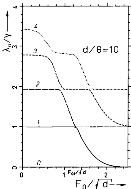
Fig. 11.46. The ratio \lambda_n/\gamma for d/\Theta = 10 as a function of F_0/\sqrt{d} in the limit \gamma \rightarrow 0 . The critical force F_{01}/\sqrt{d} = 4/\pi is also indicated
