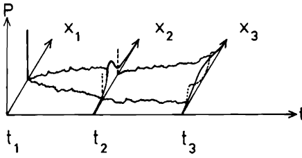
Fig. 2.2. Transition probabilities at times t_2 and t_3 , with sharp initial value at time t_1 . For two typical values the transition probabilities at t_3 , which start at t_2 with a sharp value, are shown by a broken line. Two typical realizations of the stochastic variable \xi(t) are also indicated
