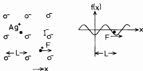
Fig. 11.4. Highly movable \text{Ag}^+ ions in the nearly fixed iodide lattice and the corresponding potential in one dimension
