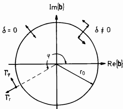
Fig. 12.13. Explanation of the enhancement of the linewidth factor due to detuning
