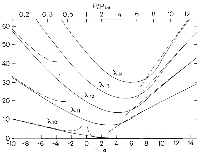
Fig. 12.6. The first five eigenvalues \lambda_{1n} as a function of the pump parameter a and as a function of the power output P/P_{\text{thr}} , respectively (solid line). The following asymptotic expansions for large positive and negative pump parameters, which can be obtained by a perturbation of the linearized equations, are also shown (dashed line):
