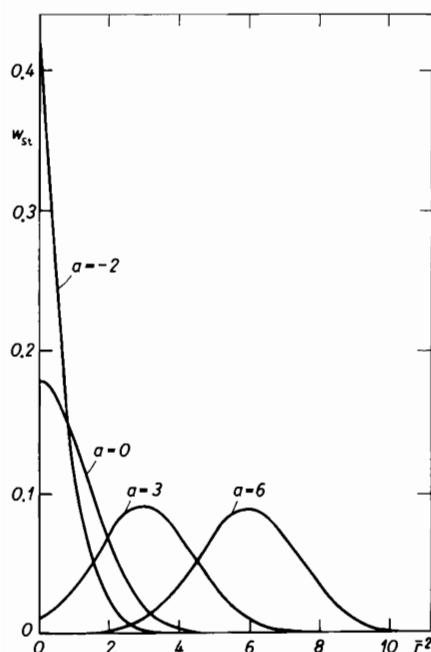
Fig. 12.3. The stationary distribution (12.45) as a function of the normalized intensity \bar{I} = \bar{r}^2 for various pump parameters a
