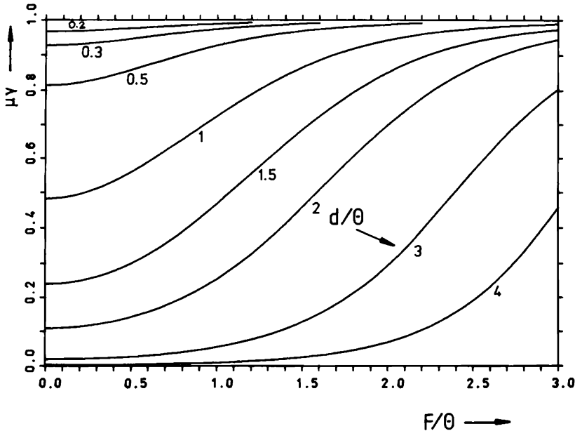
Fig. 11.20. The mobility times the damping constant as a function of F/\Theta for various amplitudes of d/\Theta of the cosine potential f(x) = -d \cos x and for \gamma/\sqrt{\Theta} = 1
