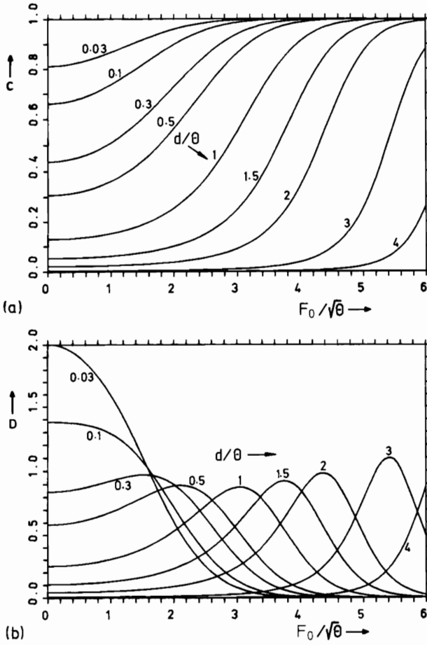
Fig. 11.18. The first expansion coefficients C (a) and D (b) of the mobility times damping constant as a function of the external force F_0/\sqrt{\theta} = F/(\gamma/\theta) for different amplitudes of the cosine potential (11.103)
