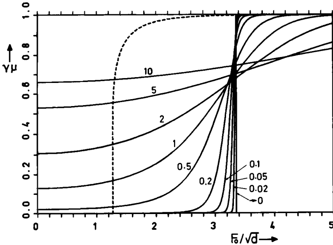
Fig. 11.27. The mobility times the damping constant of the running solution for the noiseless case ( dotted line ) and the mobility \mu times the damping constant \gamma as a function of the external force F_0/\sqrt{d} in the low-friction limit including noise for various temperatures \Theta/d ( solid lines ). For \Theta/d \geq 0.1 (11.136) was used and for \Theta/d \leq 0.1 , approximation (11.194)
