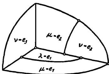
Figure 1. Confocal surfaces of the second order.
