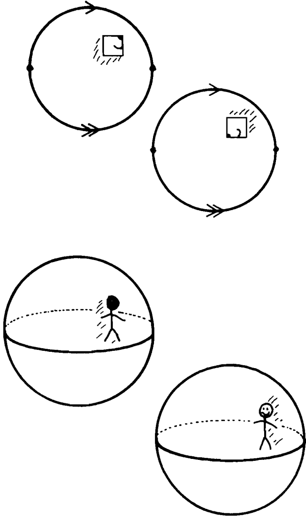
Figure 14.2 A two-sphere may be represented topologically as two disks with edges glued together. Similarly, a three-sphere may be represented topologically as two solid balls with surfaces glued together.
