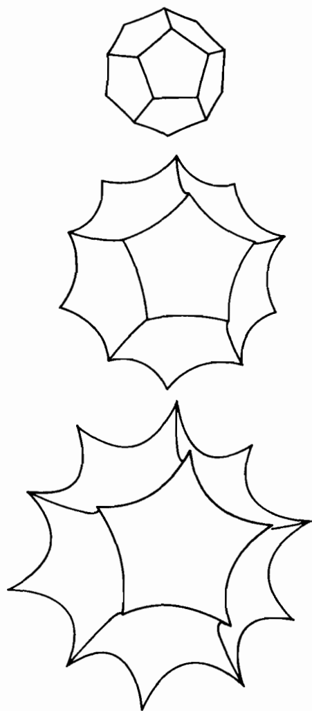
Figure 16.2 Let a dodecahedron expand in hyperbolic space until its corners are the right size to all fit together at a single point. The angles shown here are accurate, but in hyperbolic space itself the dodecahedron's faces do not bend inward.
