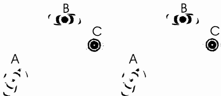
Figure 21.2 In a multiply connected universe images of galaxies repeat in a regular pattern.
