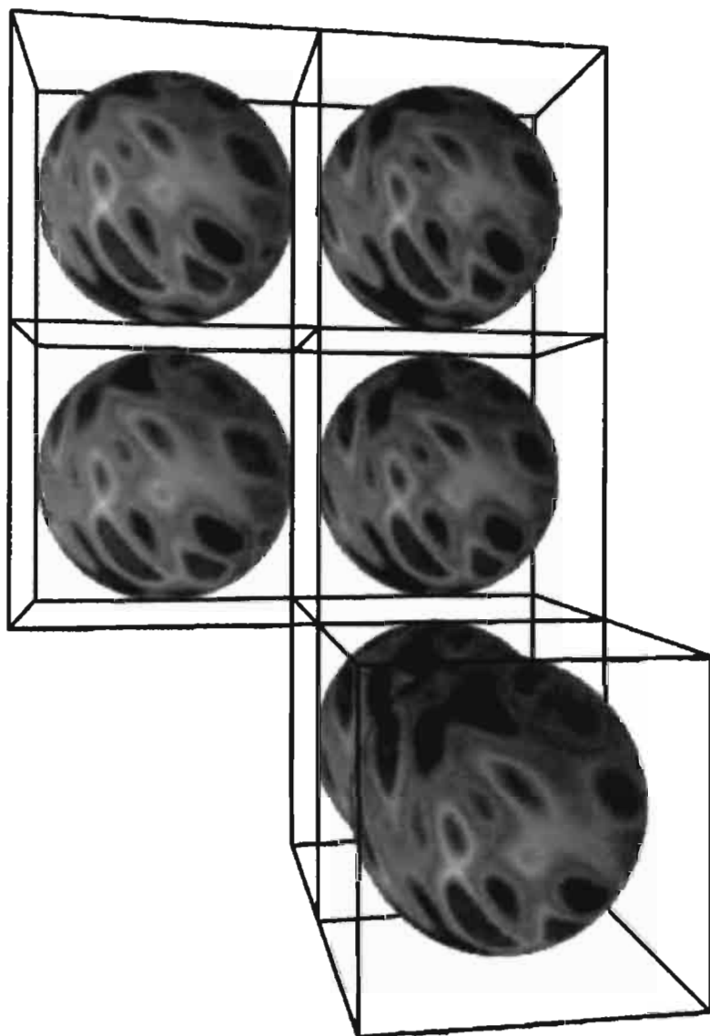
Figure 22.7 If the universe is too big, then the last scattering surface does not intersect itself.
