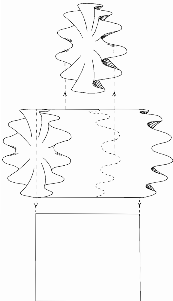
Figure 18.2 A vertical cross-section of H^2 \times S^1 has Euclidean geometry but a horizontal cross-section has hyperbolic geometry. By the way, the horizontal slices should really be stacked up in a different dimension than the one they wrinkle into, but this picture is the best we can do with only three dimensions available.
