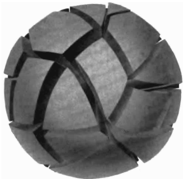
Figure 14.6 If we do not allow it to stretch, a piece of a three-sphere will split open in Euclidean space. Note that every cross-section of this split open ball is a split open disk like the one in Figure 9.8.
