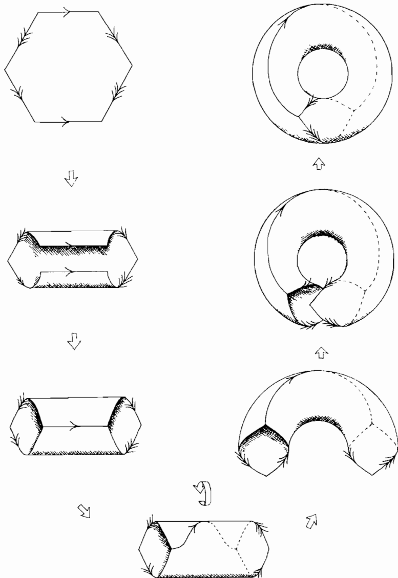
Figure 7.13 To physically glue together opposite edges of a hexagon, you must deform the hexagon into the shape of a doughnut surface. A hexagon with abstractly glued edges therefore has the same global topology as a torus.
