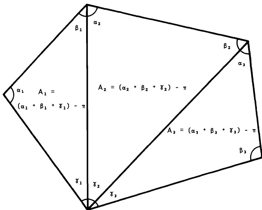
Figure 12.2 An n -gon can be divided into n - 2 triangles.
