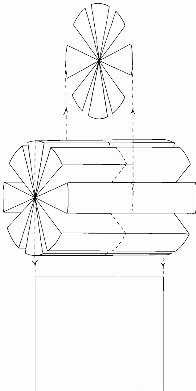
Figure 18.1 A vertical cross-section of S^2 \times S^1 has Euclidean geometry but a horizontal cross-section has elliptic geometry. A piece of S^2 \times S^1 splits vertically in Euclidean space if not allowed to stretch, but it doesn't split horizontally.
