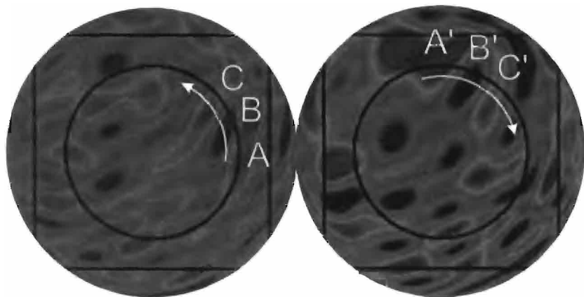
One of the pairs of circles in a quarter-turn manifold matches with a 90^\circ offset.
