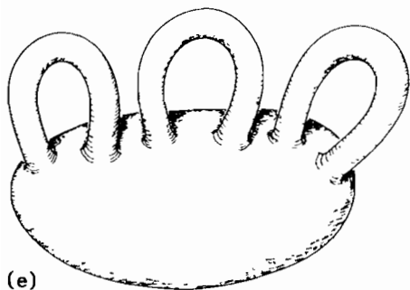
Figure 3.2 Which surfaces have the same topology?
