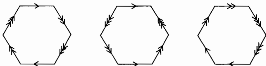
Figure 7.18 Which of these surfaces have cone points?
