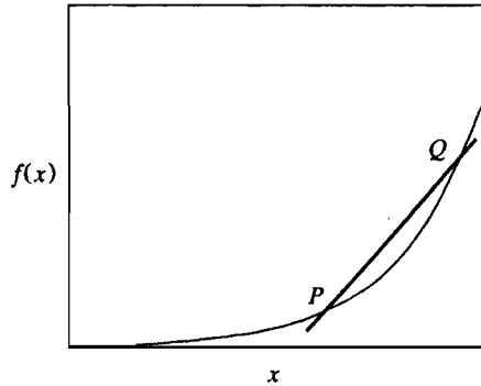
Figure 3.4. The graph of a convex function.
