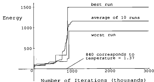
Simulated Annealing results for the permanent 14:40 problem
