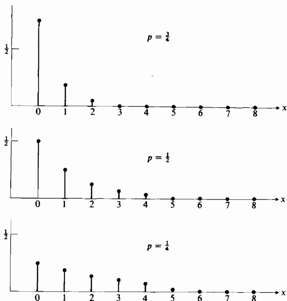
FIGURE 7 Geometric densities.
