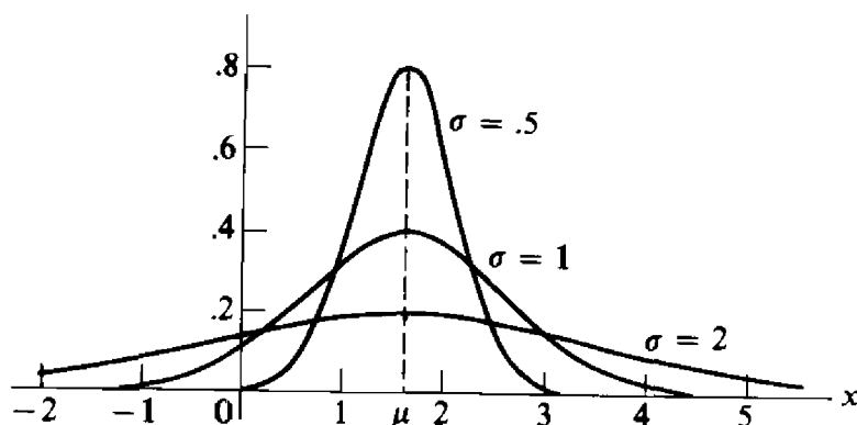
FIGURE 9 Normal densities.
