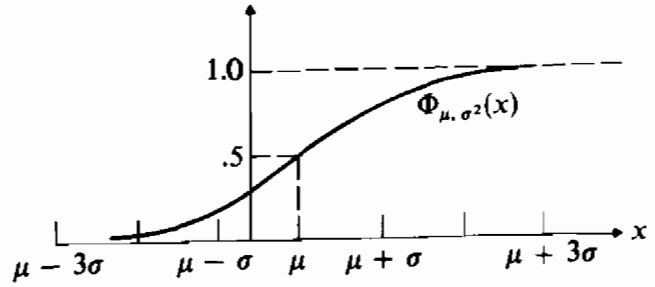
FIGURE 10 Normal cumulative distribution function.
