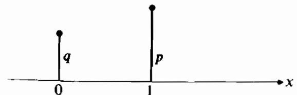
FIGURE 2 Bernoulli density.
