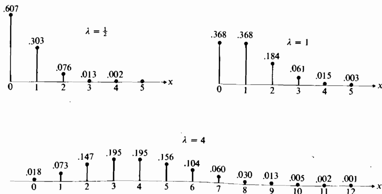
FIGURE 5 Poisson densities.
