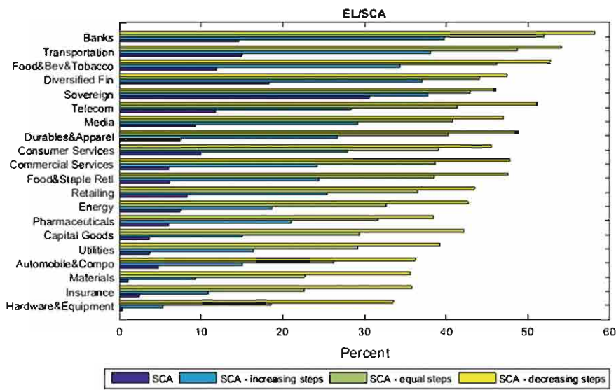
Fig. 6.9 EL/SCA with respect to different SCA methods. XFGEEESC
