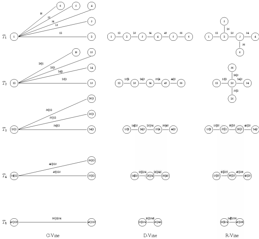
Fig. 13.2 Vine tree structures of C-vine, D-vine and R-vine
