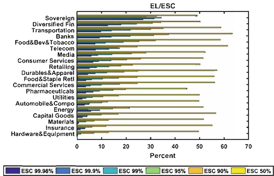
Fig. 6.10 Expected loss/risk ratio for the expected shortfall contribution at different quantiles. XFGEEESC
