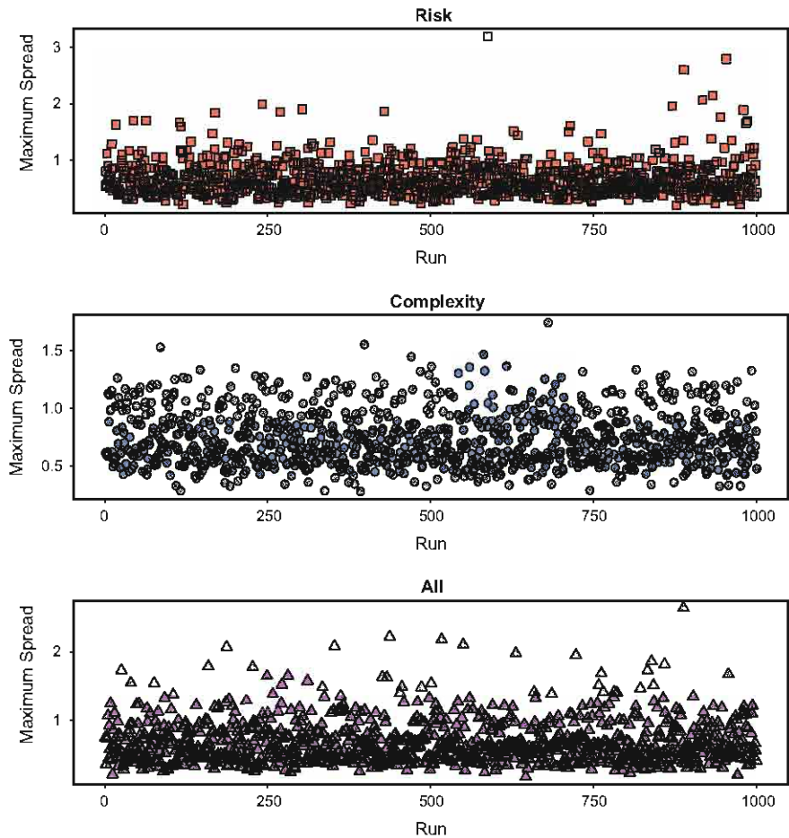
Fig. 12.18 Maximum spread among projections \mathbf{X}_1 \mathbf{w} for 1000 randomly chosen \mathbf{w}
