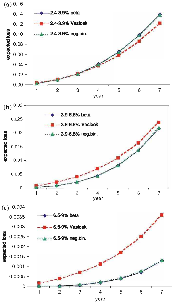
Fig. 11.5 Comparison of term structures of expected losses in tranches two, three and four with different underlying loss distributions under the constraint of matching the first two moments
