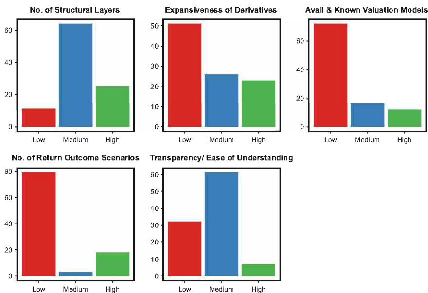
Fig. 12.2 Histograms of complexity factor scores
