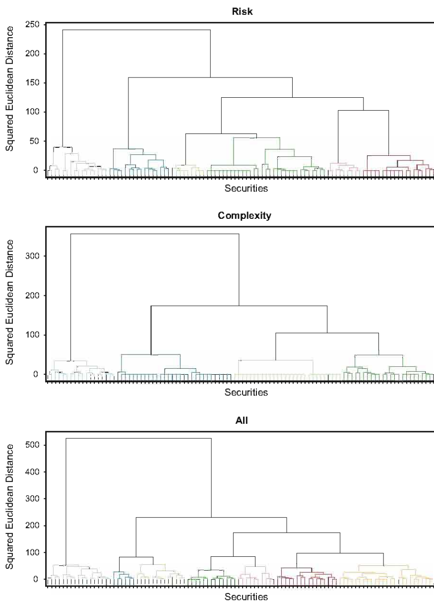
Fig. 12.3 Dendrograms of cluster analysis. Ward algorithm using Euclidean distances. Clusters formed below a threshold of 60 are coloured
