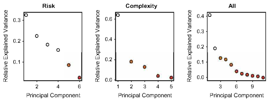
Fig. 12.4 Fraction of variance explained by each of the principal components
