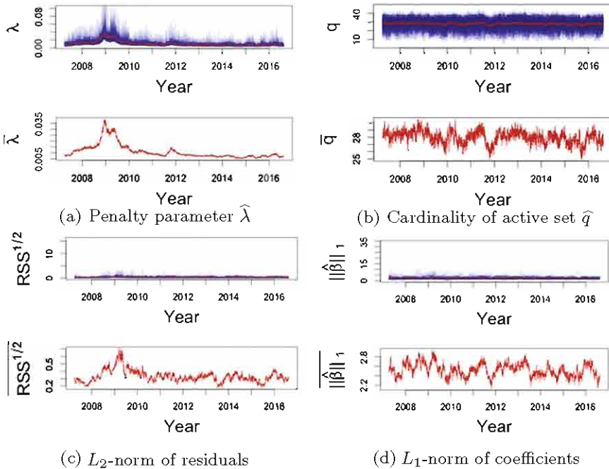
Fig. 17.7 Time series of \hat{\lambda}_k (blue) and other model characteristics and their respective averages (red) when fitted to given dataset, moving windows of length 63. QXFGTVP_FRM
