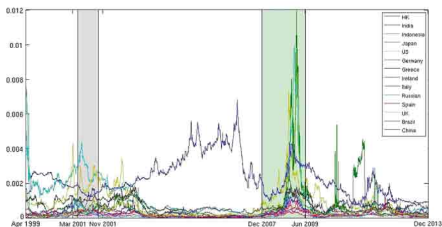
Fig. 10.1 Time series plot of the 14 economies CVI data. Gray shadow is the Dot Com bubble period and light green shadow is the Sub Prime crisis
