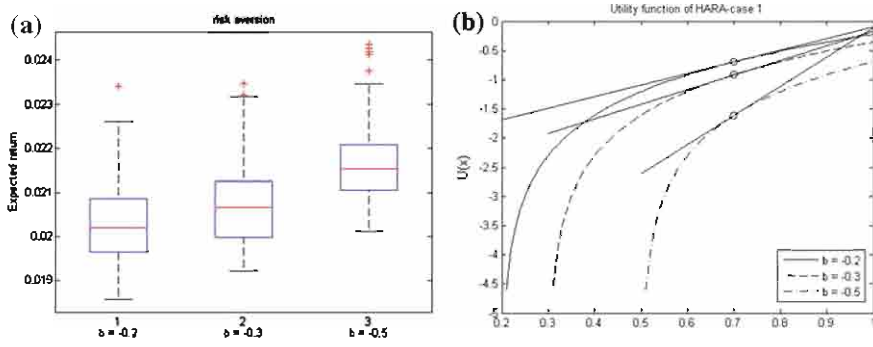
Fig. 3.4 a Boxplots of the optimal expected returns obtained by solving (3.2) with a generating function of the SRM defined in (3.9), where b = -0.2, -0.3 and -0.5 . b The corresponding utility functions for b = -0.2, -0.3 and -0.5 . XFGexp_rtn_SRM
