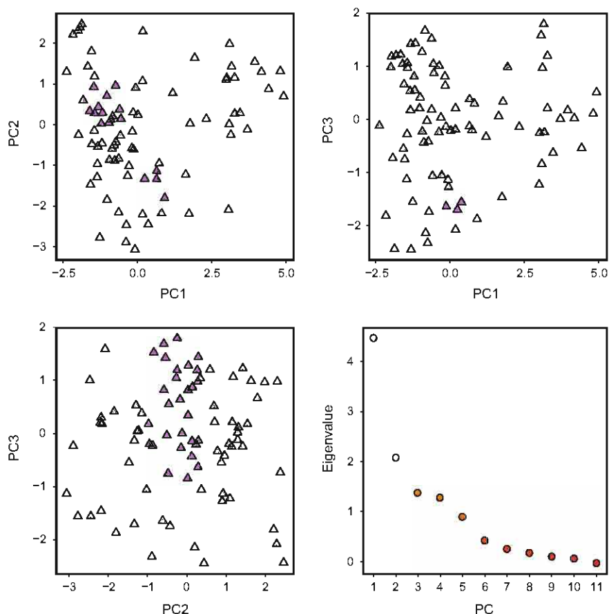
Fig. 12.8 The first three PCs derived from the PCA of the risk and complexity factors plotted against each other ( top left , top right , and bottom left ) and the eigenvalues of the polychoric correlation matrix of risk and complexity factors ( bottom right )
