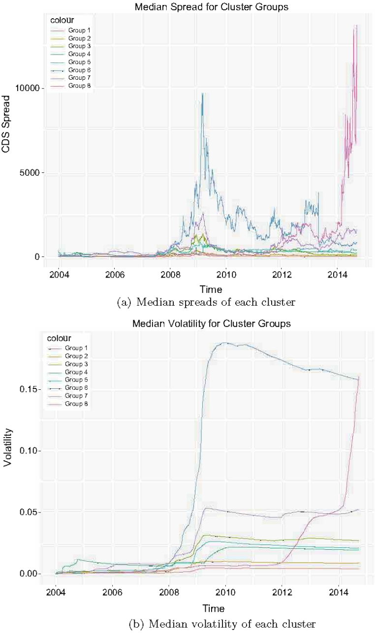
Fig. 7.4 Time plots of the median spreads and volatility for each cluster based on results of the proposed market-based credit rating
