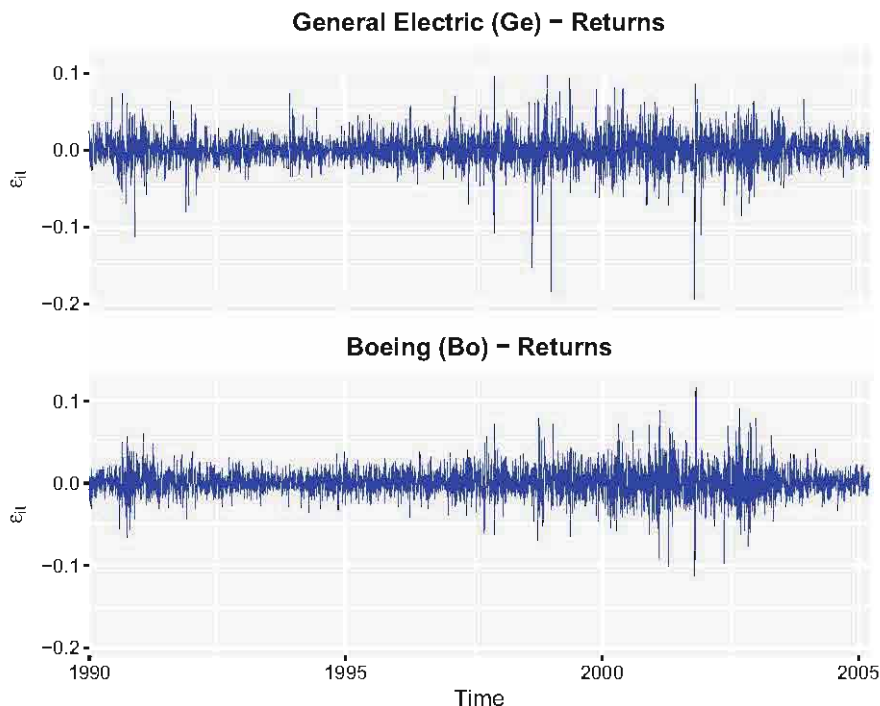
Fig. 1.3 Returns for General Electric and Boeing
