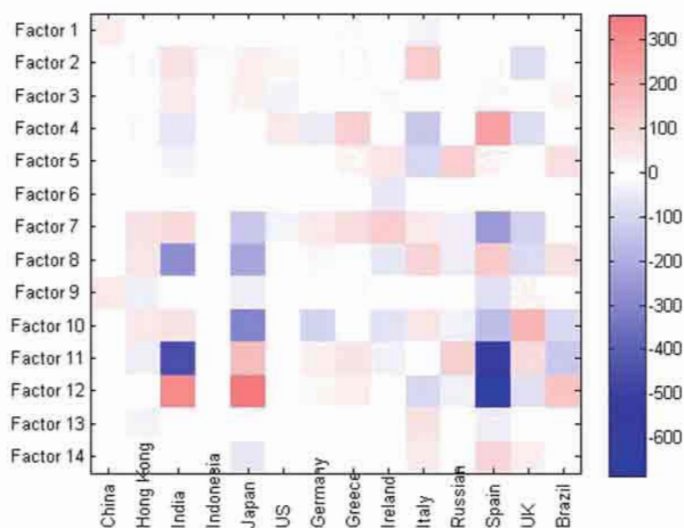
Fig. 10.4 Loading Matrix: Mar 2001–Nov 2001(Dot Corn bubble)
