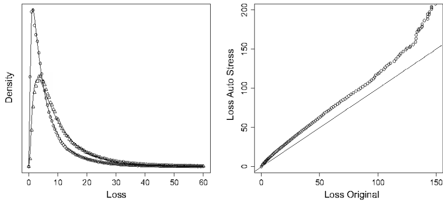
Fig. 9.3 Left graph Density plots of original (circles) and stressed (triangles) loss distributions, together with fitted Vasicek curves. Right graph QQ plot of original against stressed loss distribution
