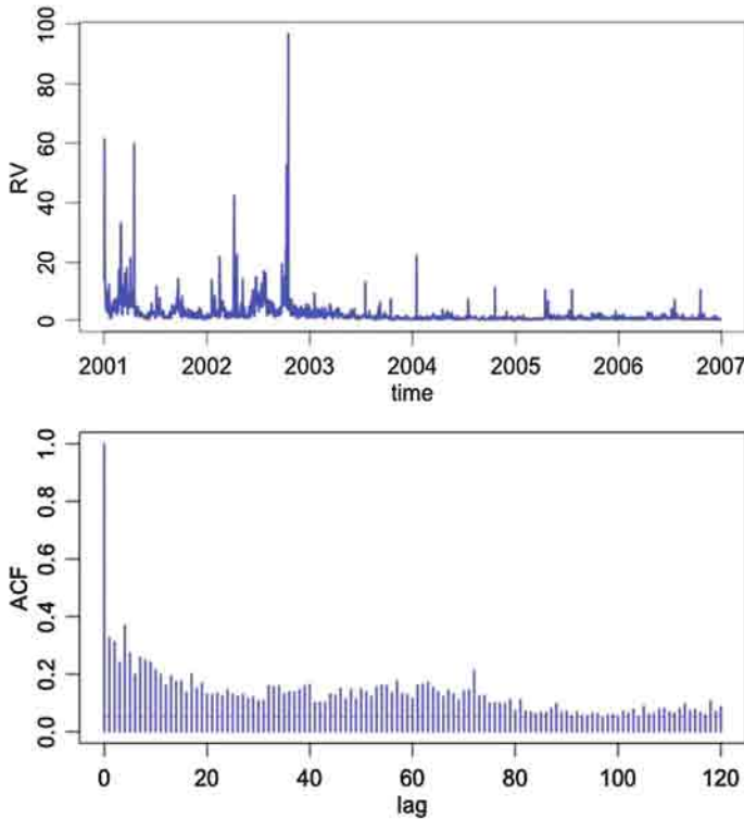
Fig. 14.3 Time evolution and sample autocorrelation function of the realized volatility for IBM, 2001–2006. XPGrvtsacf
