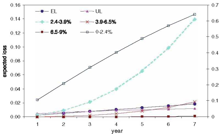
Fig. 11.4 Term structure of expected losses in tranches where the parameters of Beta-distribution ( \alpha = 0.315878 , \beta = 121.176 ) are chosen such that EL and UL match to the previous example (Vasicek-distribution with p = 0.0026 , \rho = 0.17 ). Note that in the upper plot EL[0 – 2.4%] scales with the right axis
