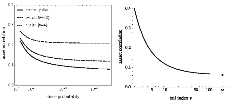
Fig. 9.5 Left Stressed asset correlation for different distribution assumptions as a function of the stress probability. Right Stressed asset correlation as a function of the tail index when the stress event is taken to the limit -\infty . Correlations are as in Fig. 9.4
