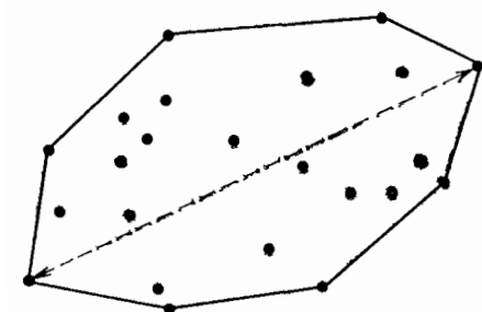
Рис. 4.19. \text{Diam}(S) = \text{Diam}(\text{CH}(S)) .
