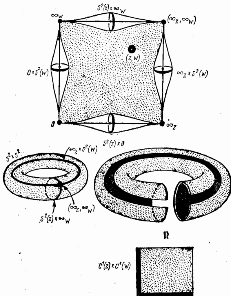
Рис. 120. (S^2 \times S^2) \setminus \{(S^2(z) \times \infty_w) \cup (\infty_z \times S^2(w))\} \cong C^2(z, w)
